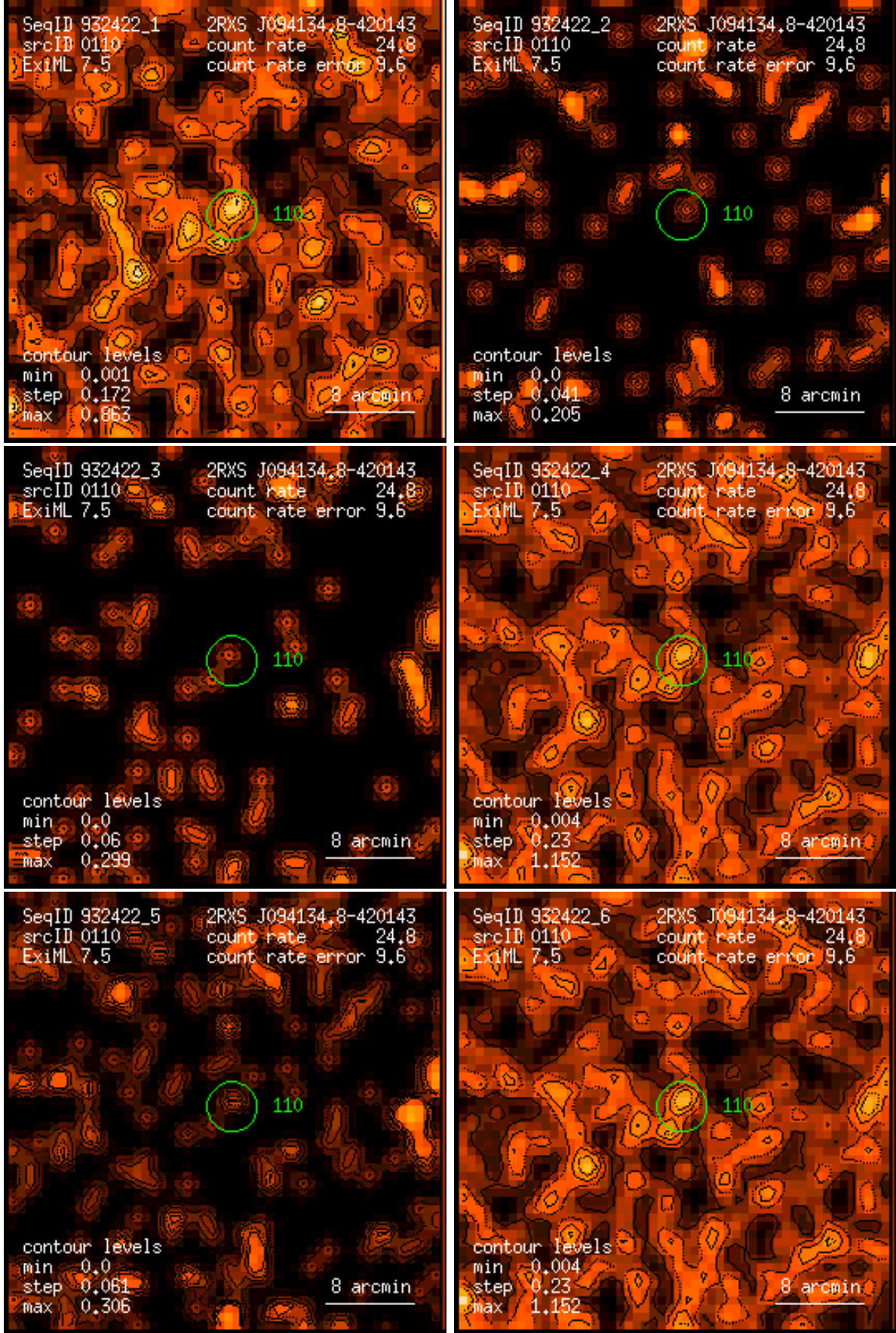
Figure 110: RASS 932422: detection 0110: band rate images, Gaussian filter: (1) PSPC channels 11 – 41, (2) 52 – 90, (3) 91 – 201, (4) 11 – 235, (5) 52 – 201, (6) 11 – 201. Broad band rates in counts/ks. Band rate contour levels in counts/ks/arcmin 2 .
