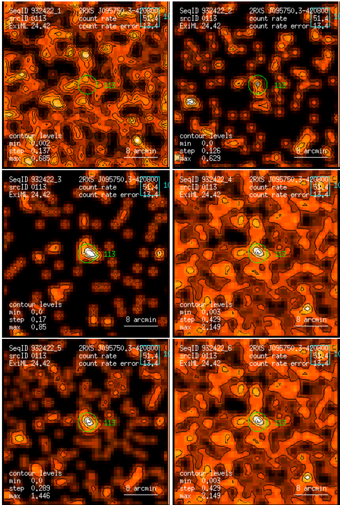
Figure 113: RASS 932422: detection 0113: band rate images, Gaussian filter: (1) PSPC channels 11 – 41, (2) 52 – 90, (3) 91 – 201, (4) 11 – 235, (5) 52 – 201, (6) 11 – 201. Broad band rates in counts/ks. Band rate contour levels in counts/ks/arcmin 2 .
