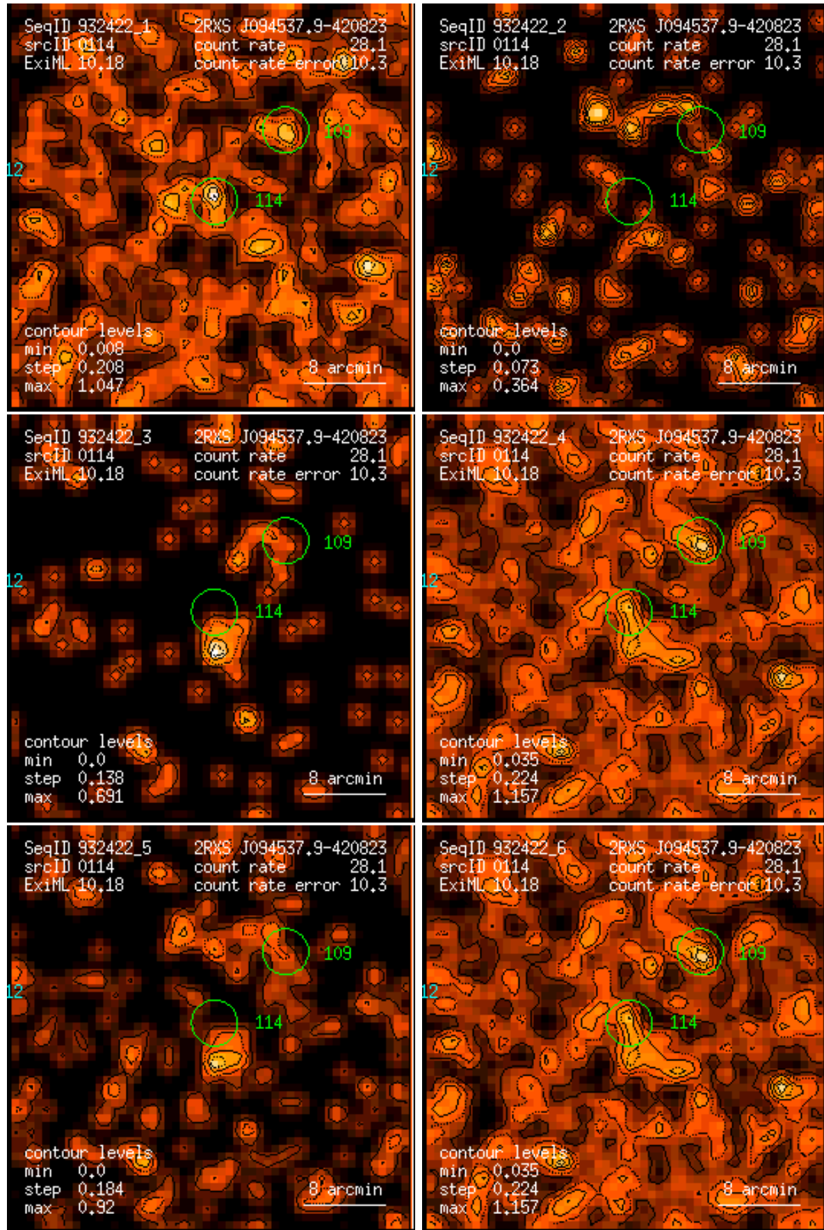
Figure 114: RASS 932422: detection 0114: band rate images, Gaussian filter: (1) PSPC channels 11 – 41, (2) 52 – 90, (3) 91 – 201, (4) 11 – 235, (5) 52 – 201, (6) 11 – 201. Broad band rates in counts/ks. Band rate contour levels in counts/ks/arcmin 2 .
