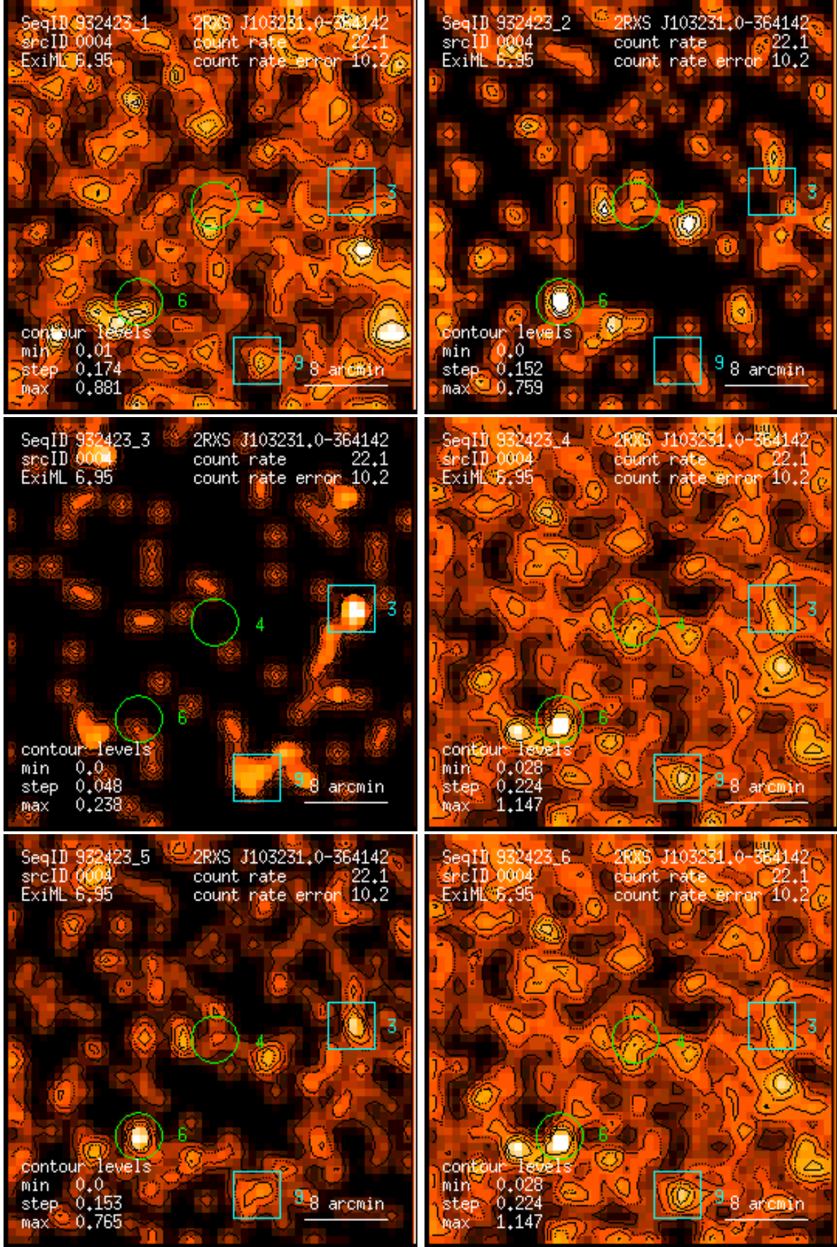
Figure 4: RASS 932423: detection 0004: band rate images, Gaussian filter: (1) PSPC channels 11 – 41, (2) 52 – 90, (3) 91 – 201, (4) 11 – 235, (5) 52 – 201, (6) 11 – 201. Broad band rates in counts/ks. Band rate contour levels in counts/ks/arcmin 2 .
