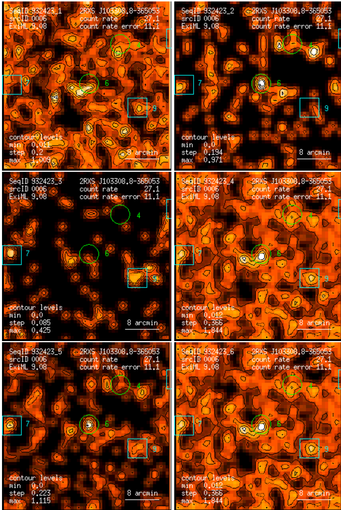
Figure 6: RASS 932423: detection 0006: band rate images, Gaussian filter: (1) PSPC channels 11 – 41, (2) 52 – 90, (3) 91 – 201, (4) 11 – 235, (5) 52 – 201, (6) 11 – 201. Broad band rates in counts/ks. Band rate contour levels in counts/ks/arcmin 2 .
