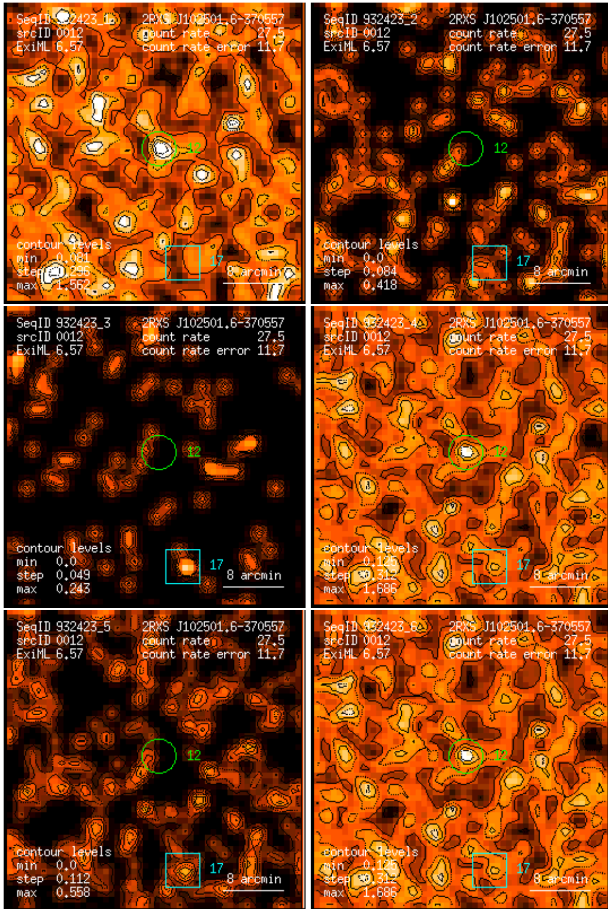
Figure 12: RASS 932423: detection 0012: band rate images, Gaussian filter: (1) PSPC channels 11 – 41, (2) 52 – 90, (3) 91 – 201, (4) 11 – 235, (5) 52 – 201, (6) 11 – 201. Broad band rates in counts/ks. Band rate contour levels in counts/ks/arcmin 2 .
