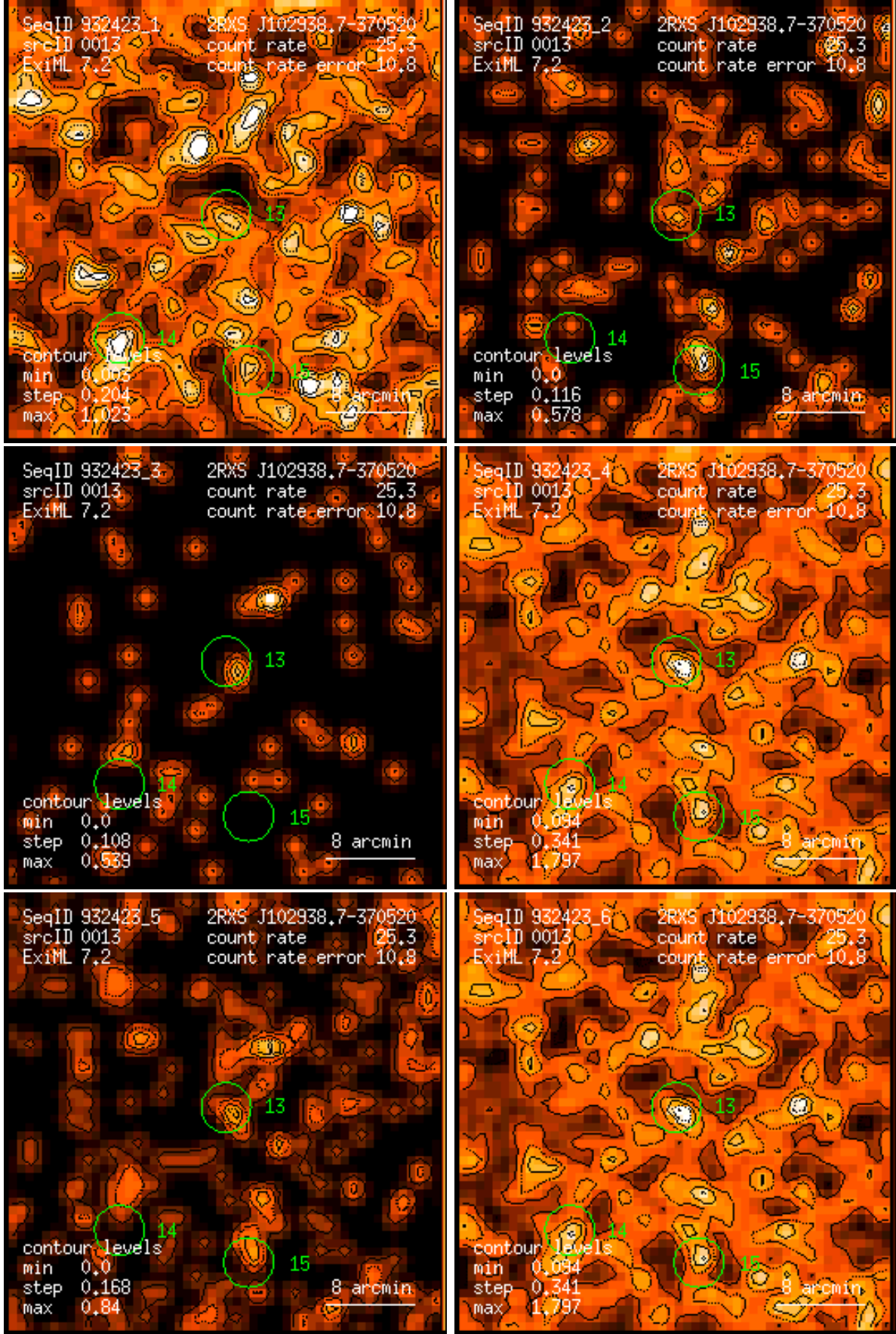
Figure 13: RASS 932423: detection 0013: band rate images, Gaussian filter: (1) PSPC channels 11 – 41, (2) 52 – 90, (3) 91 – 201, (4) 11 – 235, (5) 52 – 201, (6) 11 – 201. Broad band rates in counts/ks. Band rate contour levels in counts/ks/arcmin 2 .
