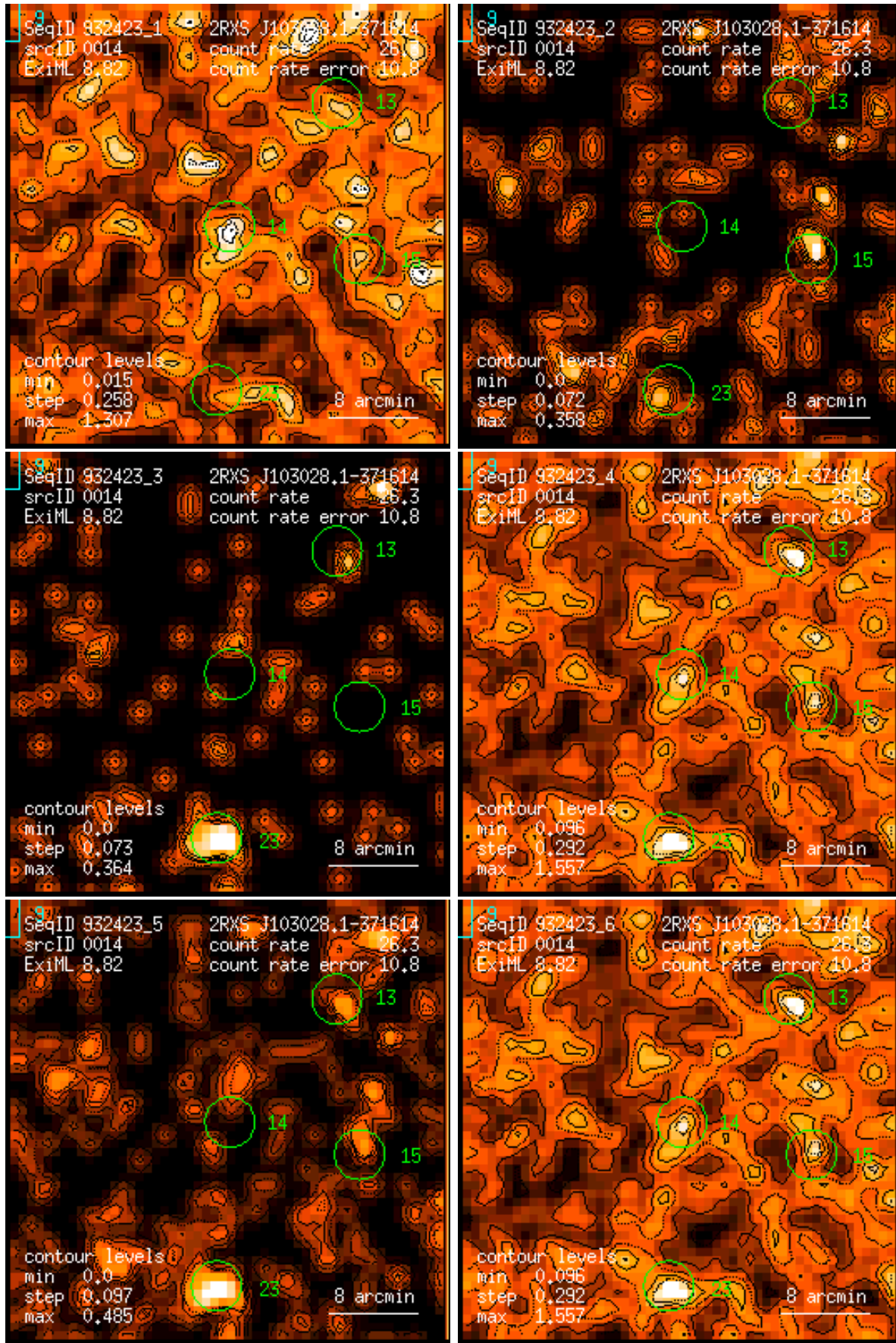
Figure 14: RASS 932423: detection 0014: band rate images, Gaussian filter: (1) PSPC channels 11 – 41, (2) 52 – 90, (3) 91 – 201, (4) 11 – 235, (5) 52 – 201, (6) 11 – 201. Broad band rates in counts/ks. Band rate contour levels in counts/ks/arcmin 2 .
