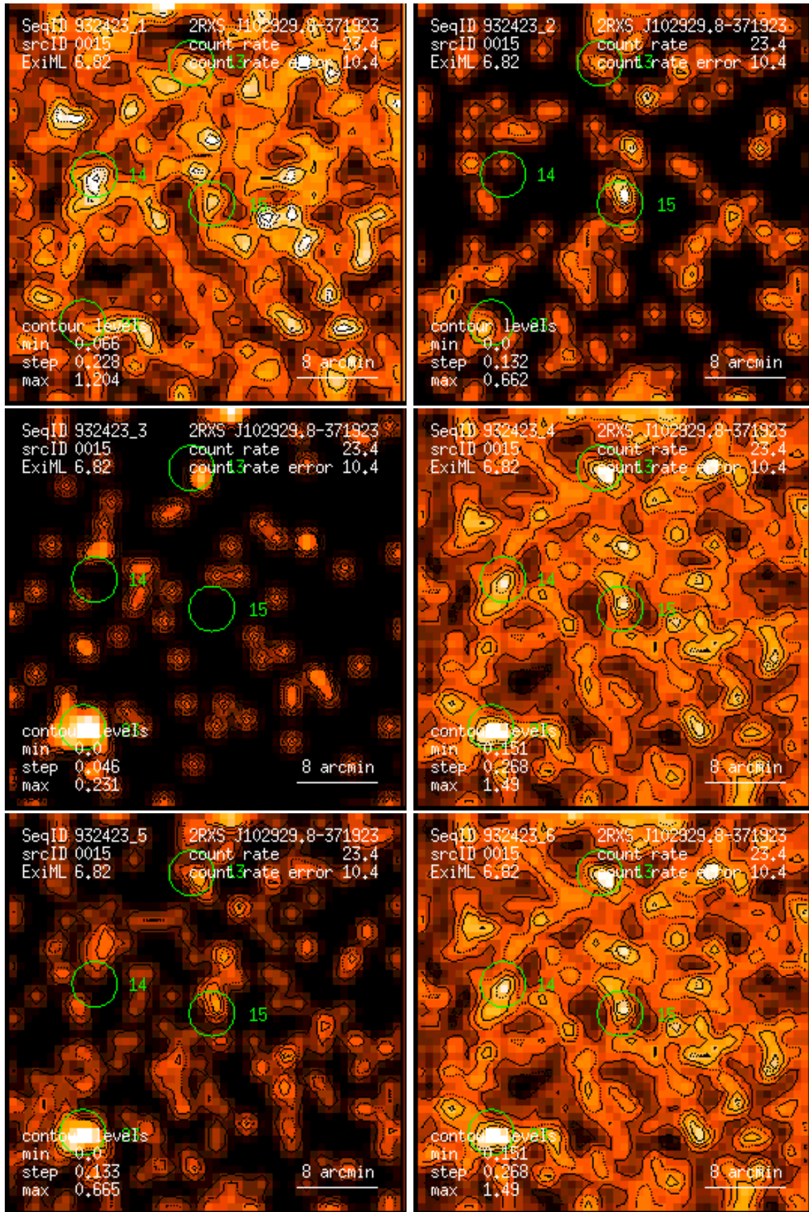
Figure 15: RASS 932423: detection 0015: band rate images, Gaussian filter: (1) PSPC channels 11 – 41, (2) 52 – 90, (3) 91 – 201, (4) 11 – 235, (5) 52 – 201, (6) 11 – 201. Broad band rates in counts/ks. Band rate contour levels in counts/ks/arcmin 2 .
