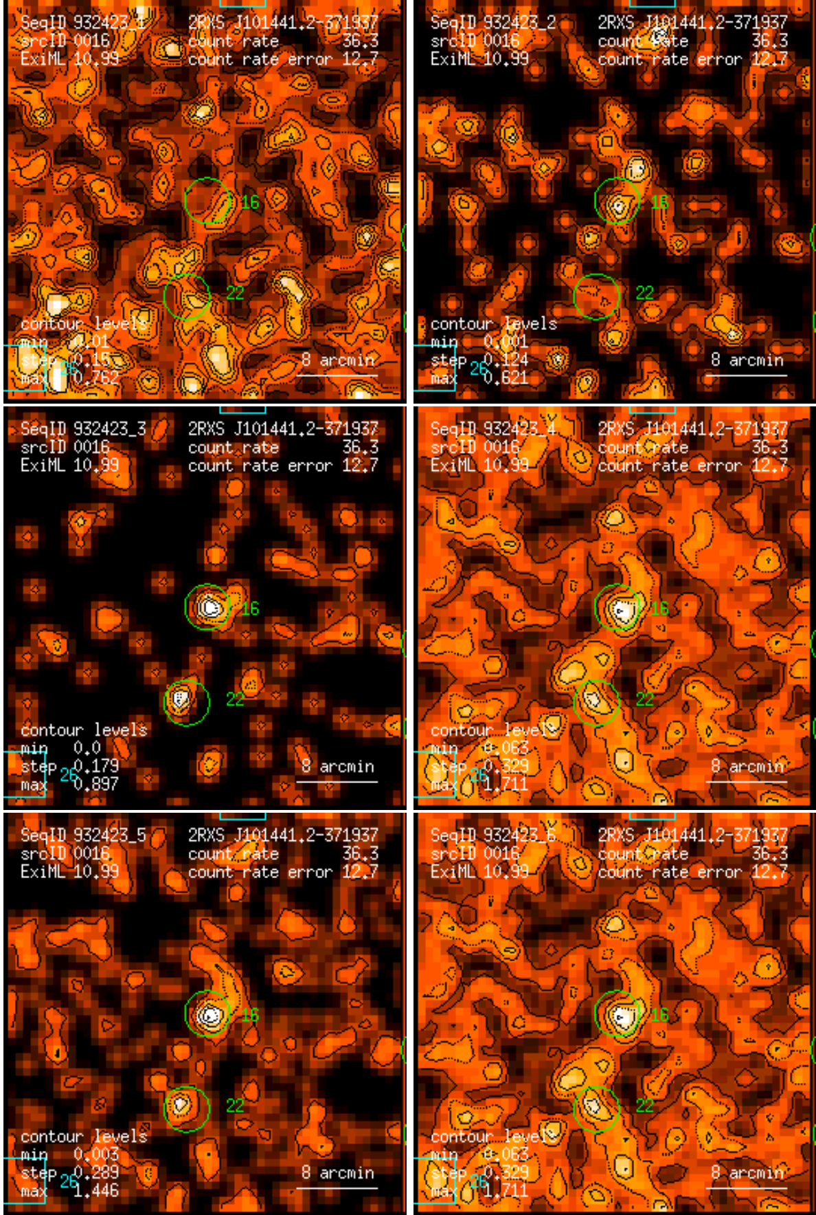
Figure 16: RASS 932423: detection 0016: band rate images, Gaussian filter: (1) PSPC channels 11 – 41, (2) 52 – 90, (3) 91 – 201, (4) 11 – 235, (5) 52 – 201, (6) 11 – 201. Broad band rates in counts/ks. Band rate contour levels in counts/ks/arcmin 2 .
