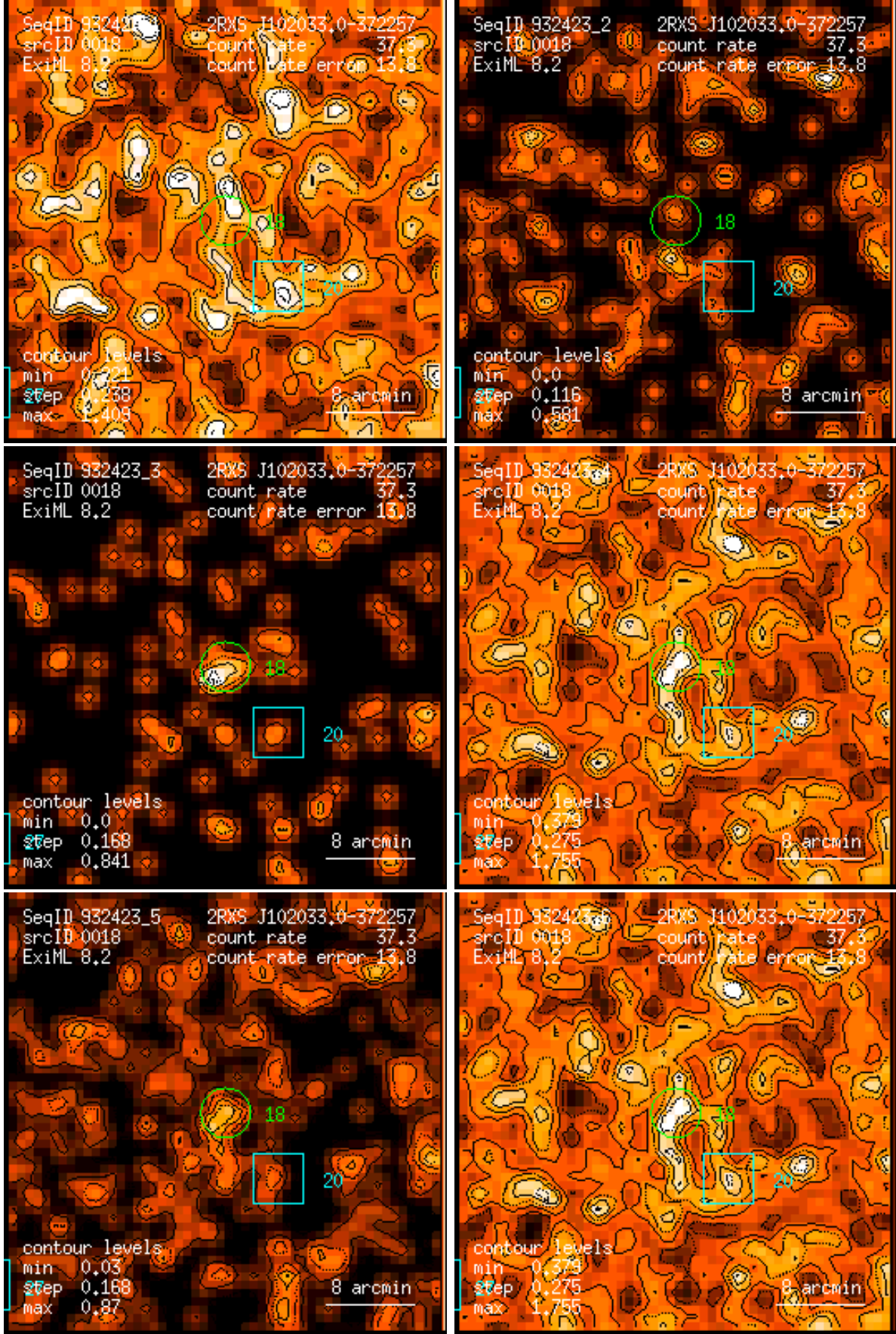
Figure 18: RASS 932423: detection 0018: band rate images, Gaussian filter: (1) PSPPC channels 11 – 41, (2) 52 – 90, (3) 91 – 201, (4) 11 – 235, (5) 52 – 201, (6) 11 – 201. Broad band rates in counts/ks. Band rate contour levels in counts/ks/arcmin 2 .
