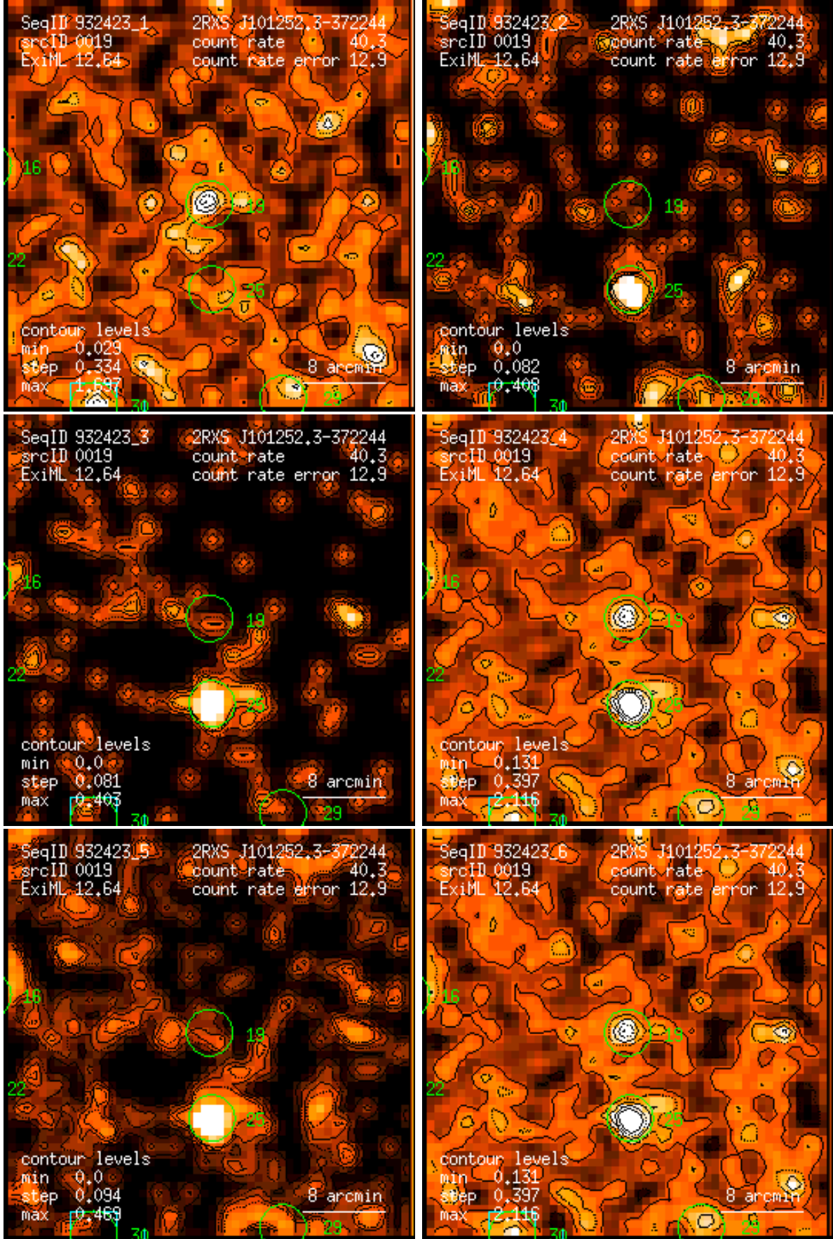
Figure 19: RASS 932423: detection 0019: band rate images, Gaussian filter: (1) PSPC channels 11 – 41, (2) 52 – 90, (3) 91 – 201, (4) 11 – 235, (5) 52 – 201, (6) 11 – 201. Broad band rates in counts/ks. Band rate contour levels in counts/ks/arcmin 2 .
