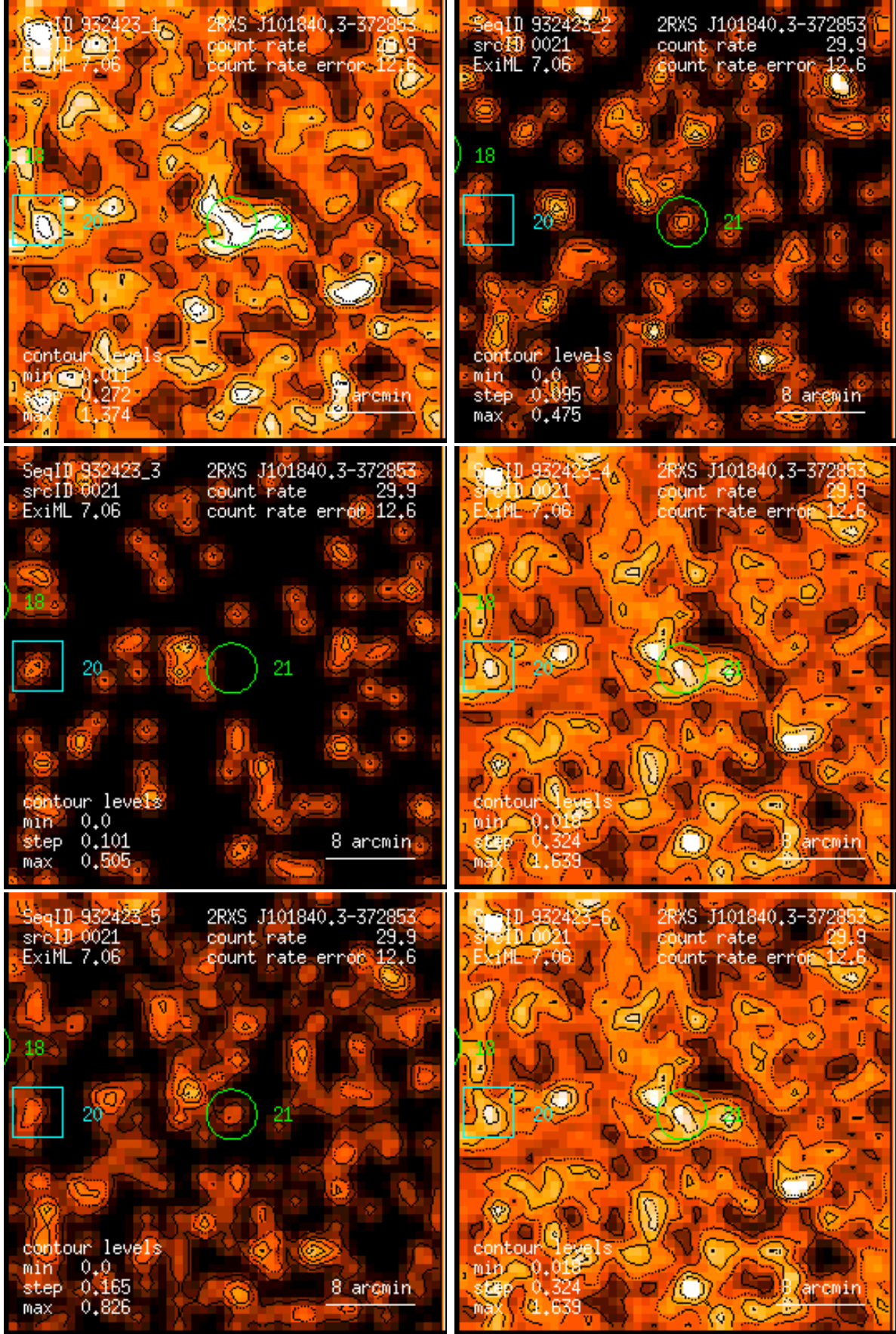
Figure 21: RASS 932423: detection 0021: band rate images, Gaussian filter: (1) PSPC channels 11 – 41, (2) 52 – 90, (3) 91 – 201, (4) 11 – 235, (5) 52 – 201, (6) 11 – 201. Broad band rates in counts/ks. Band rate contour levels in counts/ks/arcmin 2 .
