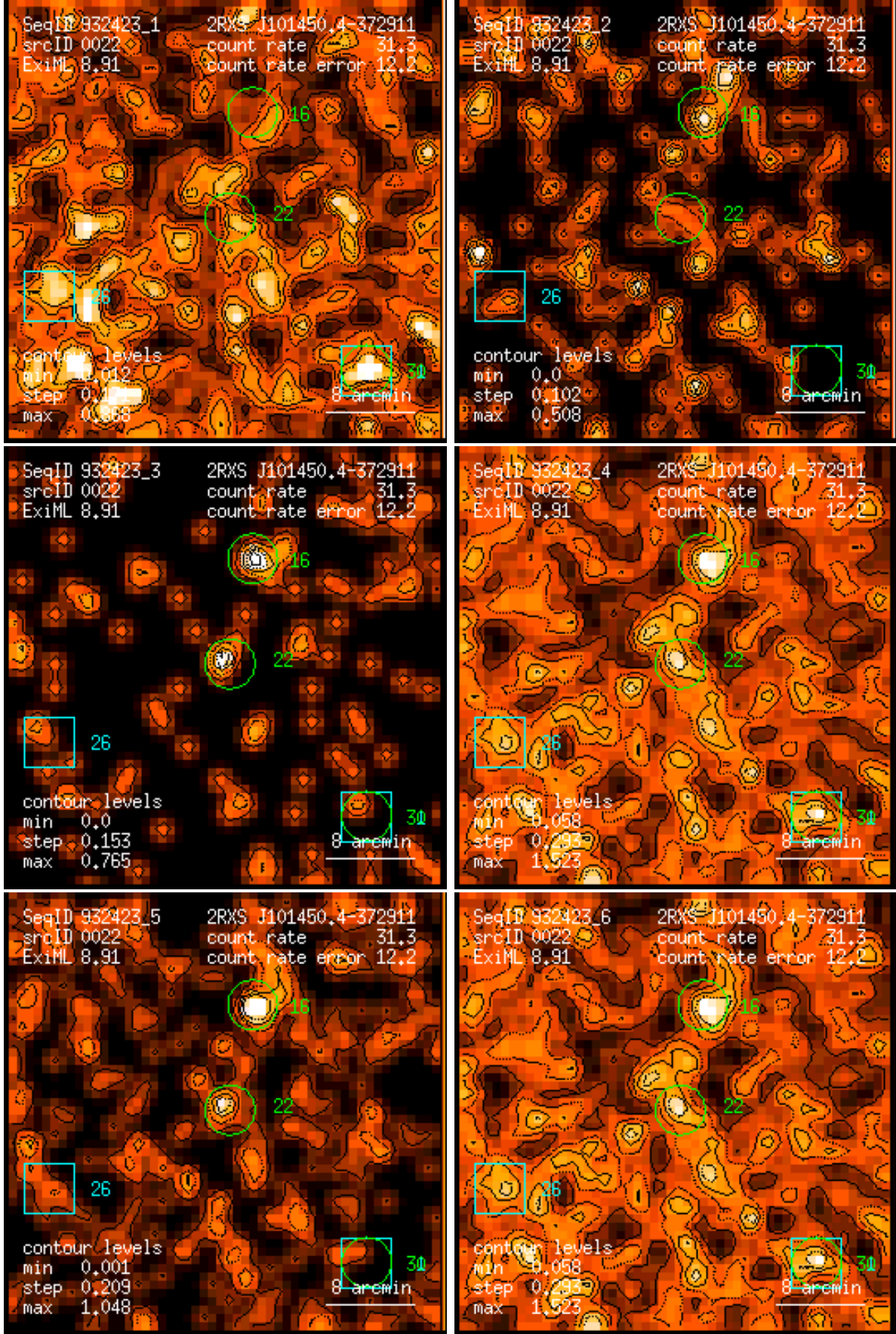
Figure 22: RASS 932423: detection 0022: band rate images, Gaussian filter: (1) PSPC channels 11 – 41, (2) 52 – 90, (3) 91 – 201, (4) 11 – 235, (5) 52 – 201, (6) 11 – 201. Broad band rates in counts/ks. Band rate contour levels in counts/ks/arcmin 2 .
