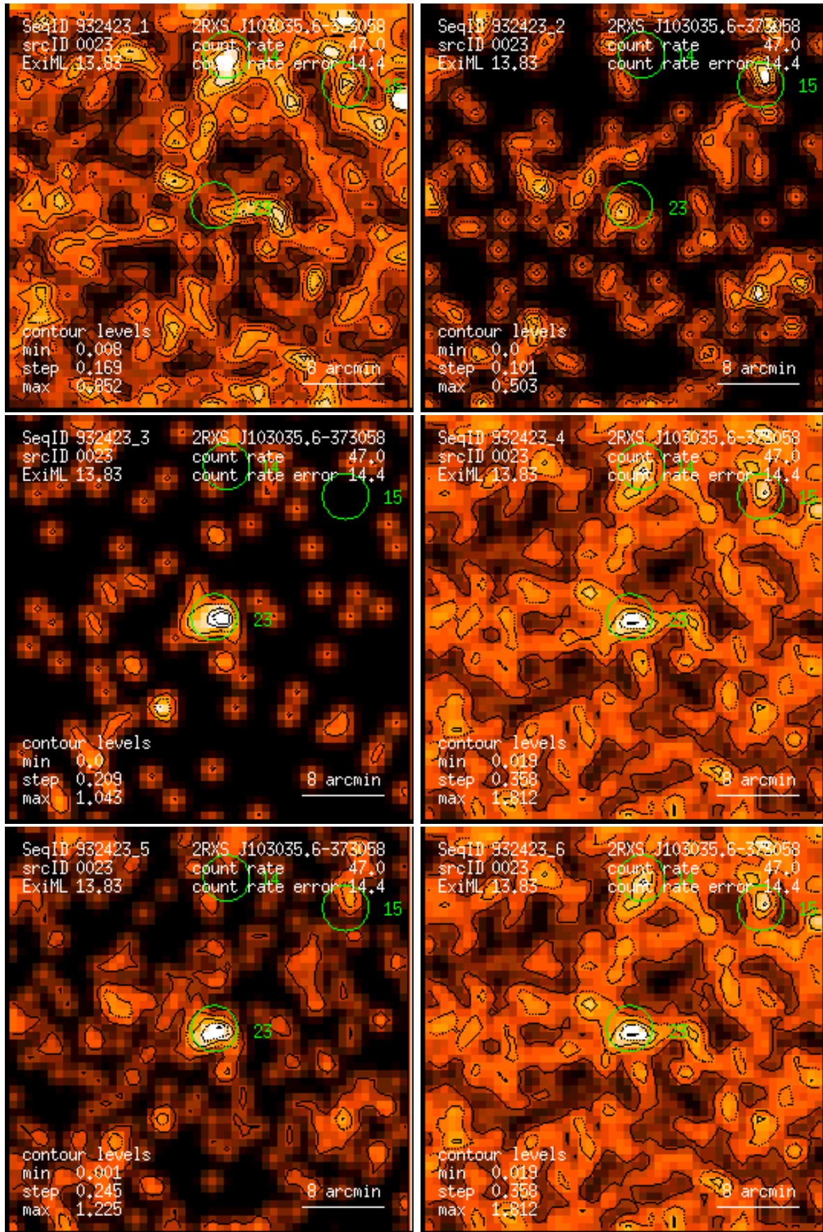
Figure 23: RASS 932423: detection 0023: band rate images, Gaussian filter: (1) PSPC channels 11 – 41, (2) 52 – 90, (3) 91 – 201, (4) 11 – 235, (5) 52 – 201, (6) 11 – 201. Broad band rates in counts/ks. Band rate contour levels in counts/ks/arcmin 2 .
