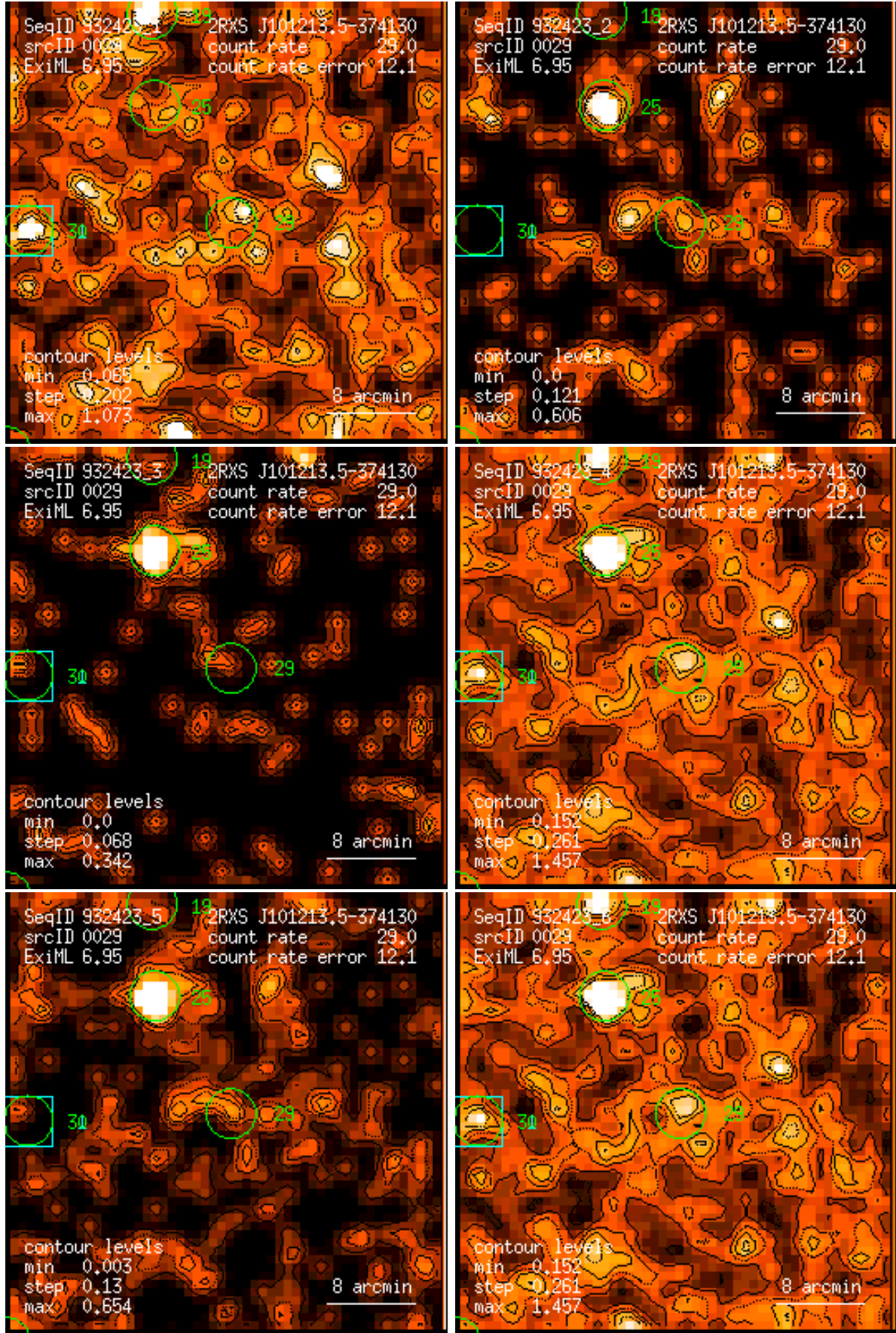
Figure 29: RASS 932423: detection 0029: band rate images, Gaussian filter: (1) PSPC channels 11 – 41, (2) 52 – 90, (3) 91 – 201, (4) 11 – 235, (5) 52 – 201, (6) 11 – 201. Broad band rates in counts/ks. Band rate contour levels in counts/ks/arcmin 2 .
