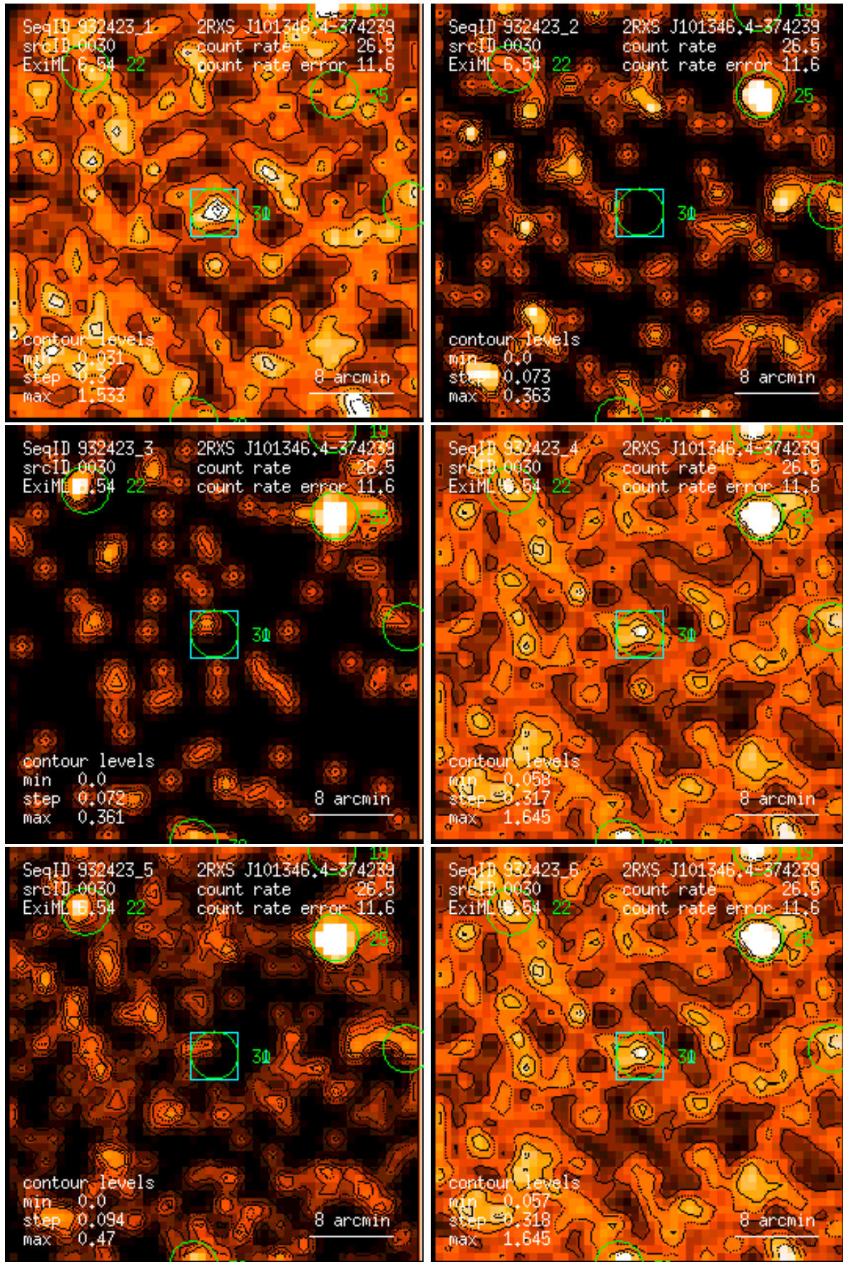
Figure 30: RASS 932423: detection 0030: band rate images, Gaussian filter: (1) PSPC channels 11 – 41, (2) 52 – 90, (3) 91 – 201, (4) 11 – 235, (5) 52 – 201, (6) 11 – 201. Broad band rates in counts/ks. Band rate contour levels in counts/ks/arcmin 2 .
