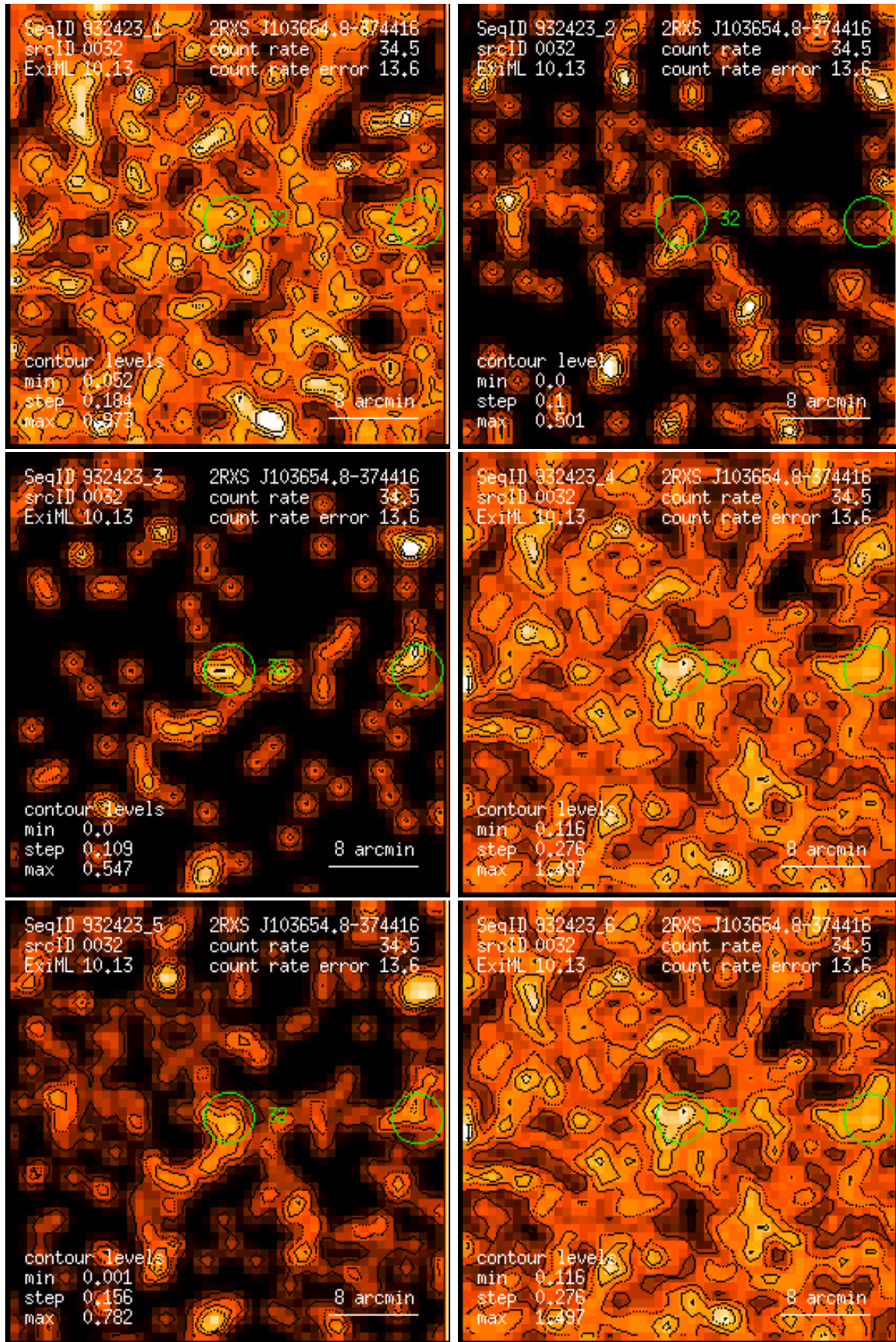
Figure 32: RASS 932423: detection 0032: band rate images, Gaussian filter: (1) PSPC channels 11 – 41, (2) 52 – 90, (3) 91 – 201, (4) 11 – 235, (5) 52 – 201, (6) 11 – 201. Broad band rates in counts/ks. Band rate contour levels in counts/ks/arcmin 2 .
