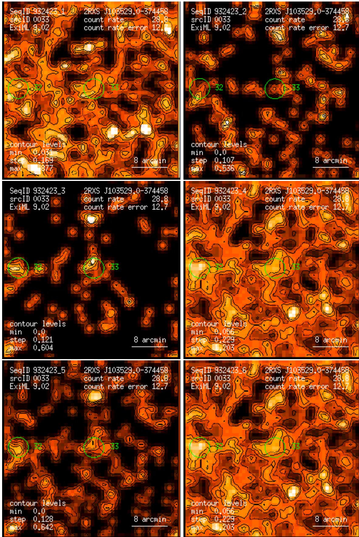
Figure 33: RASS 932423: detection 0033: band rate images, Gaussian filter: (1) PSPC channels 11 – 41, (2) 52 – 90, (3) 91 – 201, (4) 11 – 235, (5) 52 – 201, (6) 11 – 201. Broad band rates in counts/ks. Band rate contour levels in counts/ks/arcmin 2 .
