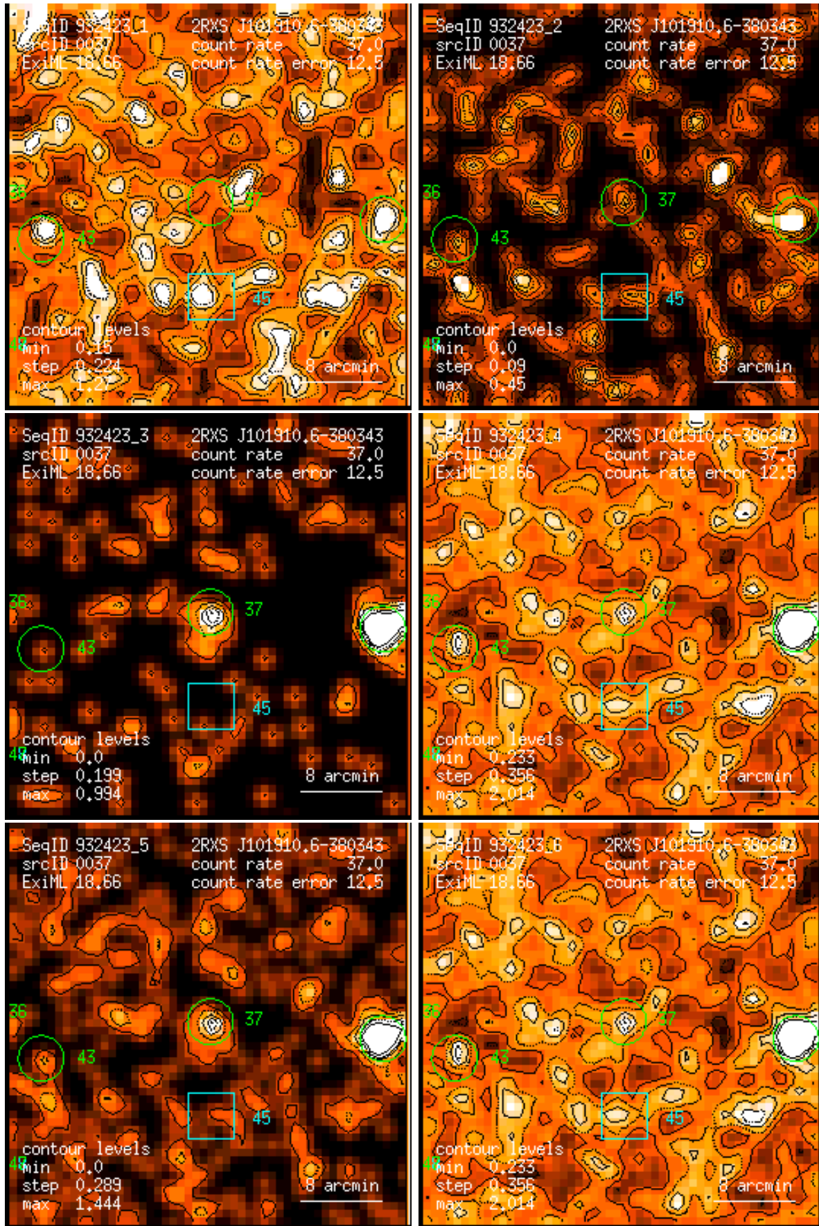
Figure 37: RASS 932423: detection 0037: band rate images, Gaussian filter: (1) PSPC channels 11 – 41, (2) 52 – 90, (3) 91 – 201, (4) 11 – 235, (5) 52 – 201, (6) 11 – 201. Broad band rates in counts/ks. Band rate contour levels in counts/ks/arcmin 2 .
