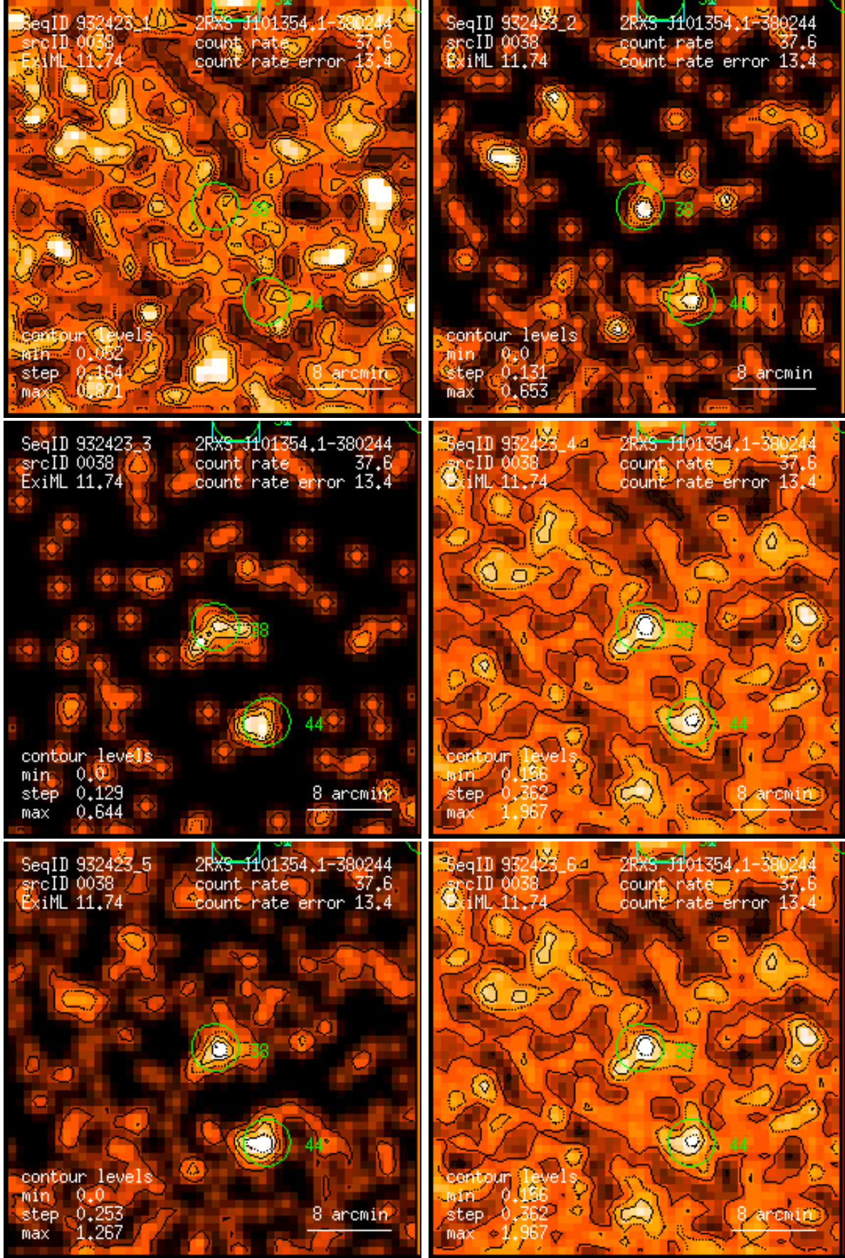
Figure 38: RASS 932423: detection 0038: band rate images, Gaussian filter: (1) PSPC channels 11 – 41, (2) 52 – 90, (3) 91 – 201, (4) 11 – 235, (5) 52 – 201, (6) 11 – 201. Broad band rates in counts/ks. Band rate contour levels in counts/ks/arcmin 2 .
