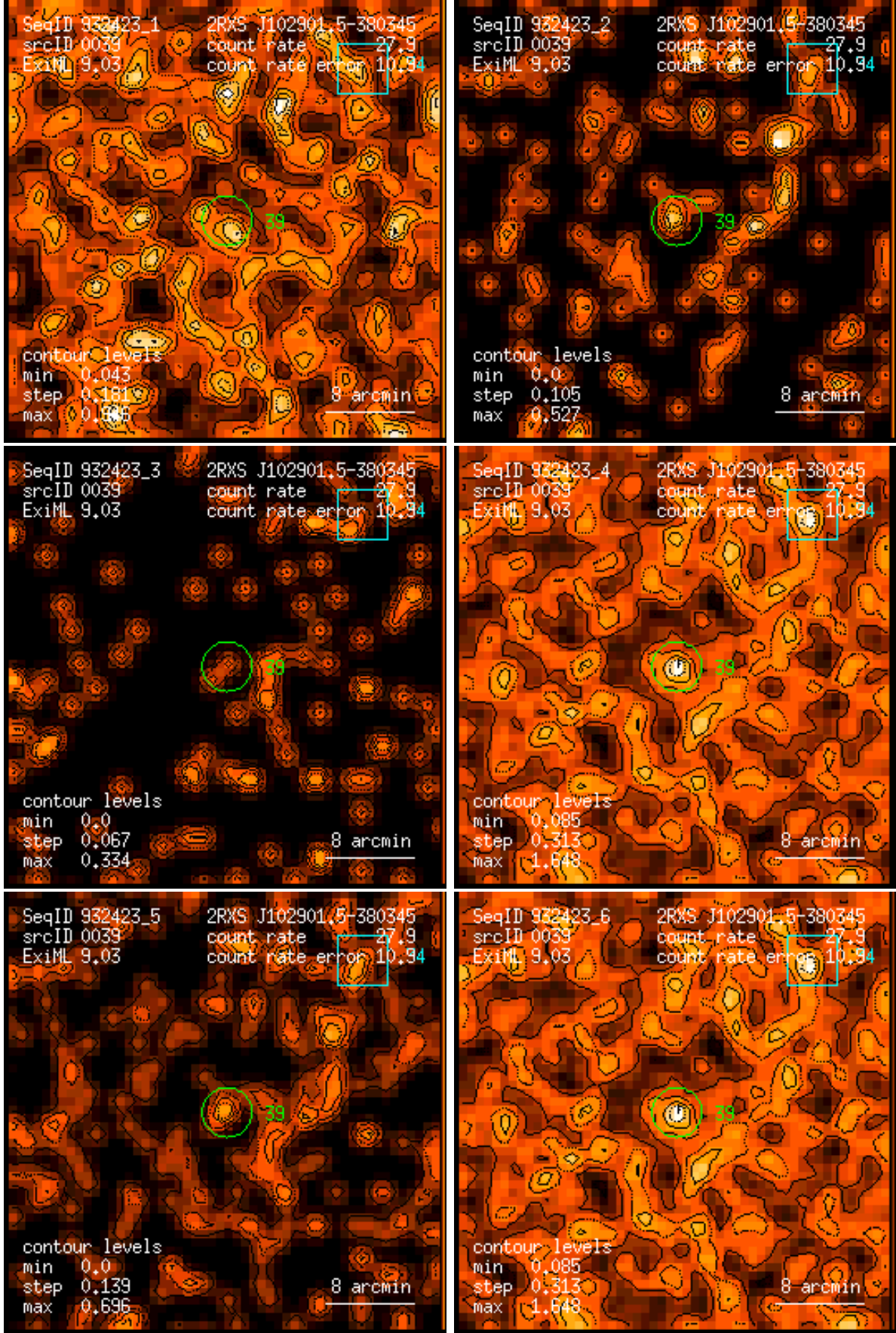
Figure 39: RASS 932423: detection 0039: band rate images, Gaussian filter: (1) PSPC channels 11 – 41, (2) 52 – 90, (3) 91 – 201, (4) 11 – 235, (5) 52 – 201, (6) 11 – 201. Broad band rates in counts/ks. Band rate contour levels in counts/ks/arcmin 2 .
