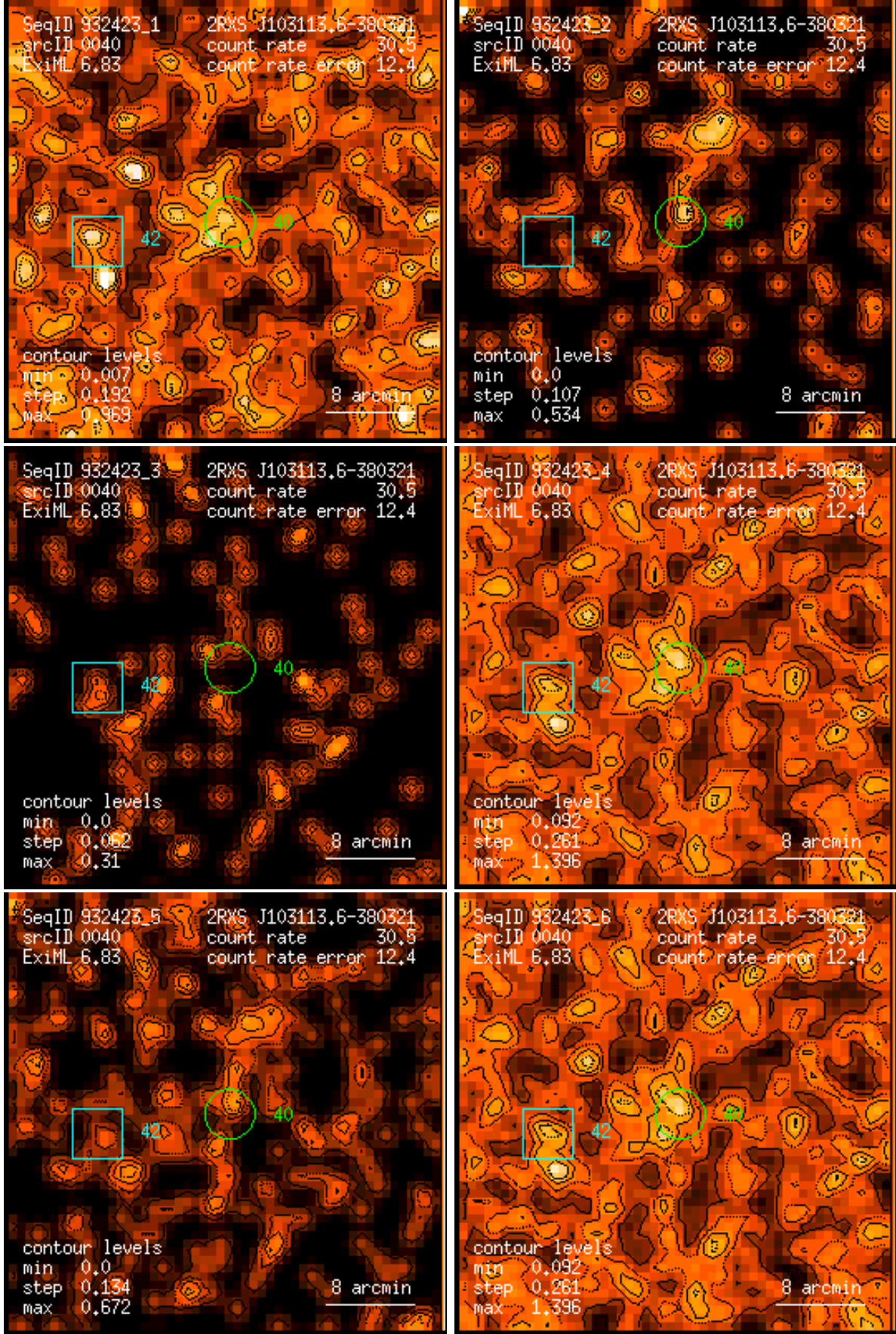
Figure 40: RASS 932423: detection 0040: band rate images, Gaussian filter: (1) PSPC channels 11 – 41, (2) 52 – 90, (3) 91 – 201, (4) 11 – 235, (5) 52 – 201, (6) 11 – 201. Broad band rates in counts/ks. Band rate contour levels in counts/ks/arcmin 2 .
