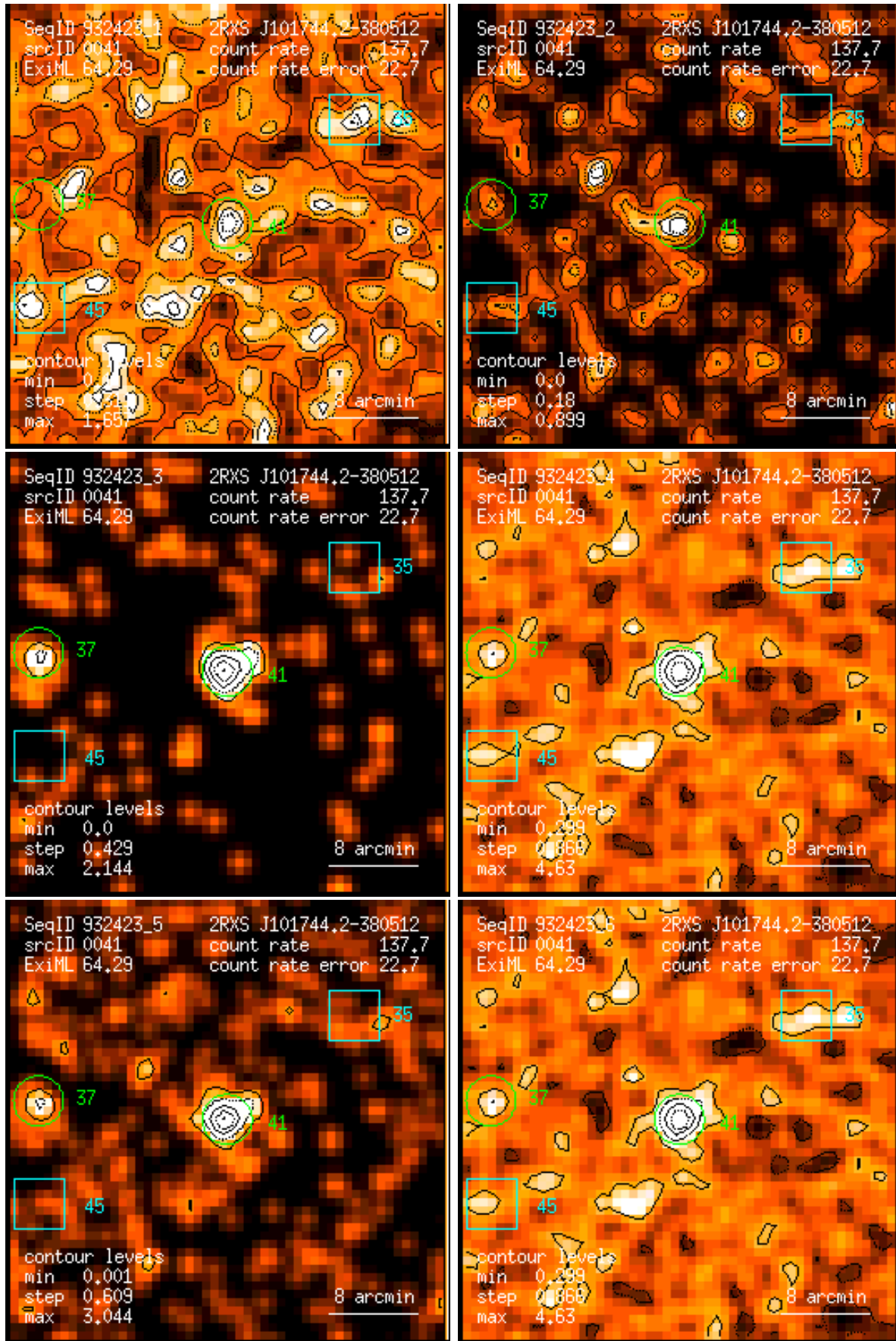
Figure 41: RASS 932423: detection 0041: band rate images, Gaussian filter: (1) PSPC channels 11 – 41, (2) 52 – 90, (3) 91 – 201, (4) 11 – 235, (5) 52 – 201, (6) 11 – 201. Broad band rates in counts/ks. Band rate contour levels in counts/ks/arcmin 2 .
