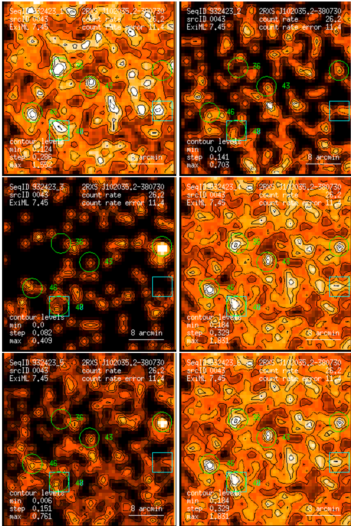
Figure 43: RASS 932423: detection 0043: band rate images, Gaussian filter: (1) PSPC channels 11 – 41, (2) 52 – 90, (3) 91 – 201, (4) 11 – 235, (5) 52 – 201, (6) 11 – 201. Broad band rates in counts/ks. Band rate contour levels in counts/ks/arcmin 2 .
