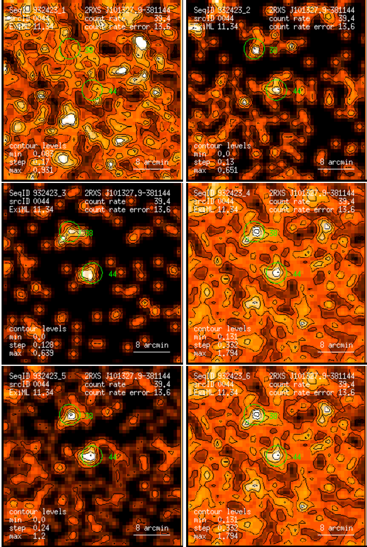
Figure 44: RASS 932423: detection 0044: band rate images, Gaussian filter: (1) PSPC channels 11 – 41, (2) 52 – 90, (3) 91 – 201, (4) 11 – 235, (5) 52 – 201, (6) 11 – 201. Broad band rates in counts/ks. Band rate contour levels in counts/ks/arcmin 2 .
