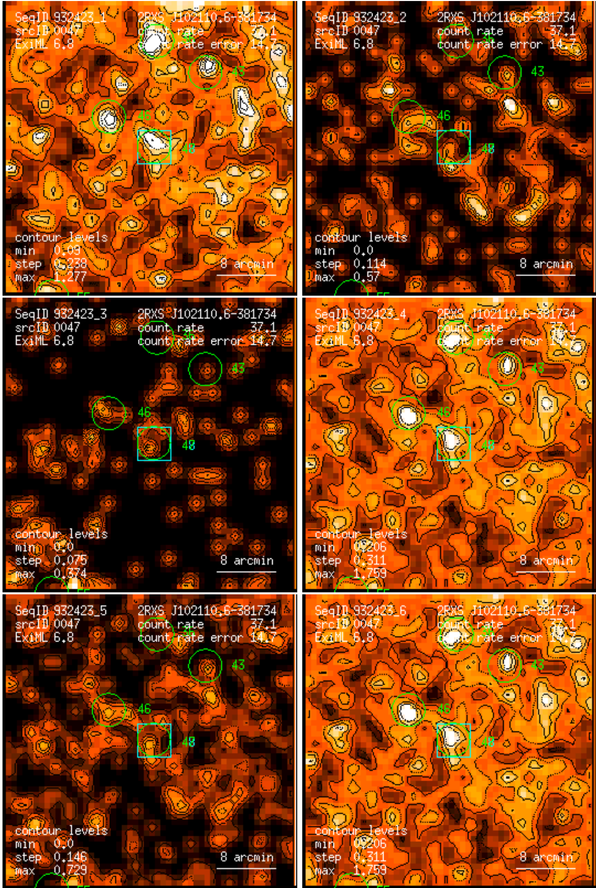
Figure 47: RASS 932423: detection 0047: band rate images, Gaussian filter: (1) PSPC channels 11 – 41, (2) 52 – 90, (3) 91 – 201, (4) 11 – 235, (5) 52 – 201, (6) 11 – 201. Broad band rates in counts/ks. Band rate contour levels in counts/ks/arcmin 2 .
