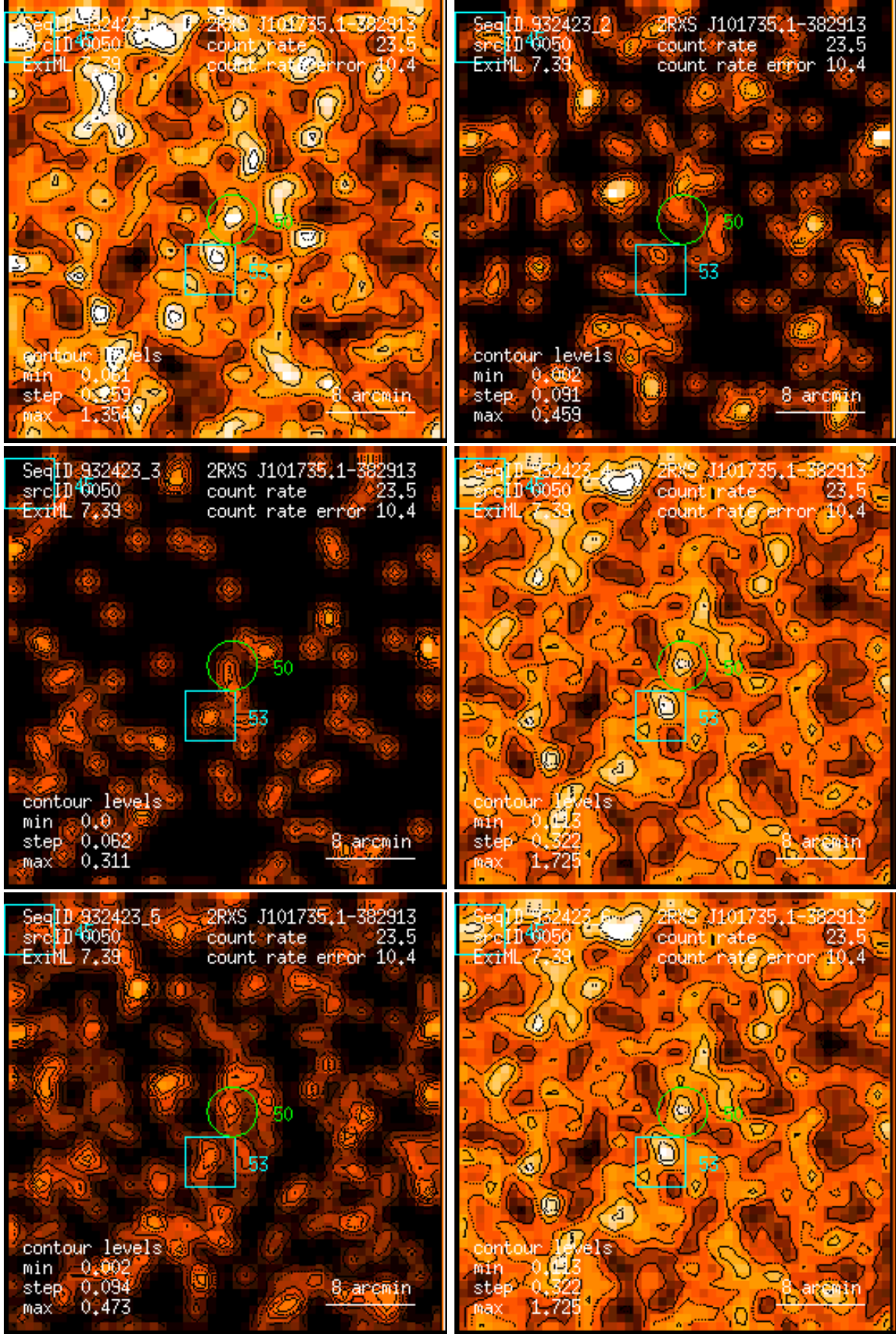
Figure 50: RASS 932423: detection 0050: band rate images, Gaussian filter: (1) PSPC channels 11 – 41, (2) 52 – 90, (3) 91 – 201, (4) 11 – 235, (5) 52 – 201, (6) 11 – 201. Broad band rates in counts/ks. Band rate contour levels in counts/ks/arcmin 2 .
