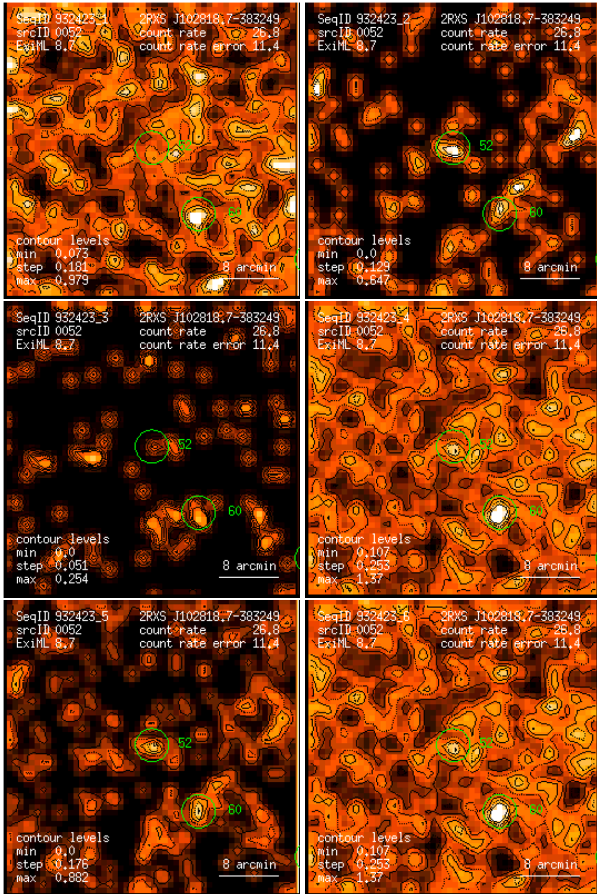
Figure 52: RASS 932423: detection 0052: band rate images, Gaussian filter: (1) PSPC channels 11 – 41, (2) 52 – 90, (3) 91 – 201, (4) 11 – 235, (5) 52 – 201, (6) 11 – 201. Broad band rates in counts/ks. Band rate contour levels in counts/ks/arcmin 2 .
