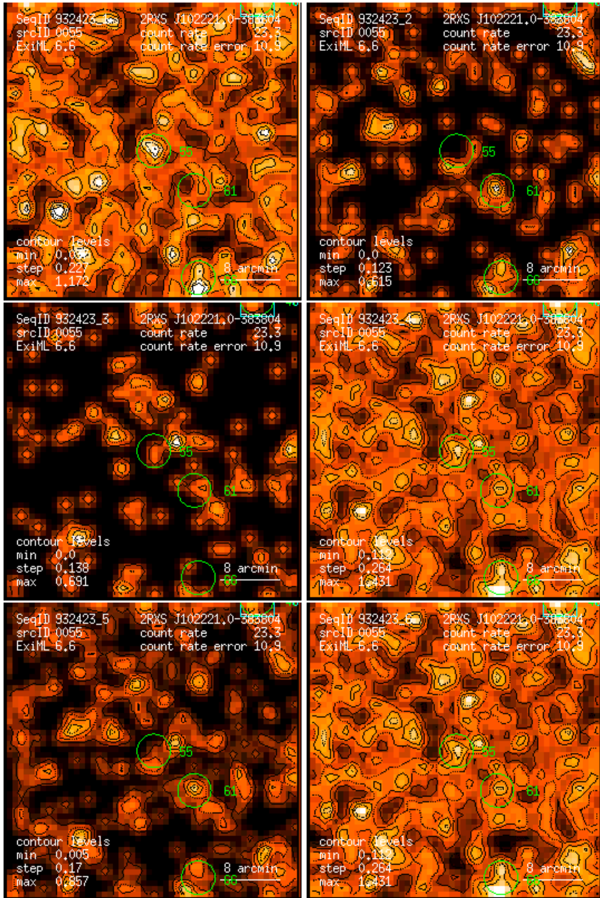
Figure 55: RASS 932423: detection 0055: band rate images, Gaussian filter: (1) PSPC channels 11 – 41, (2) 52 – 90, (3) 91 – 201, (4) 11 – 235, (5) 52 – 201, (6) 11 – 201. Broad band rates in counts/ks. Band rate contour levels in counts/ks/arcmin 2 .
