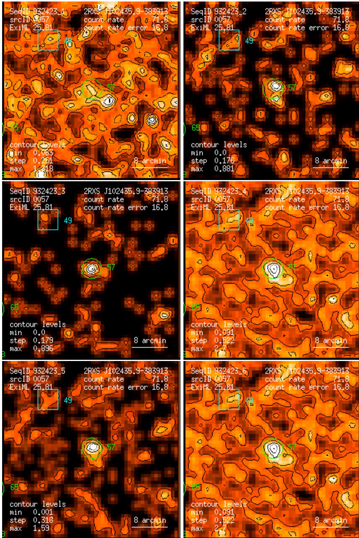
Figure 57: RASS 932423: detection 0057: band rate images, Gaussian filter: (1) PSPC channels 11 – 41, (2) 52 – 90, (3) 91 – 201, (4) 11 – 235, (5) 52 – 201, (6) 11 – 201. Broad band rates in counts/ks. Band rate contour levels in counts/ks/arcmin 2 .
