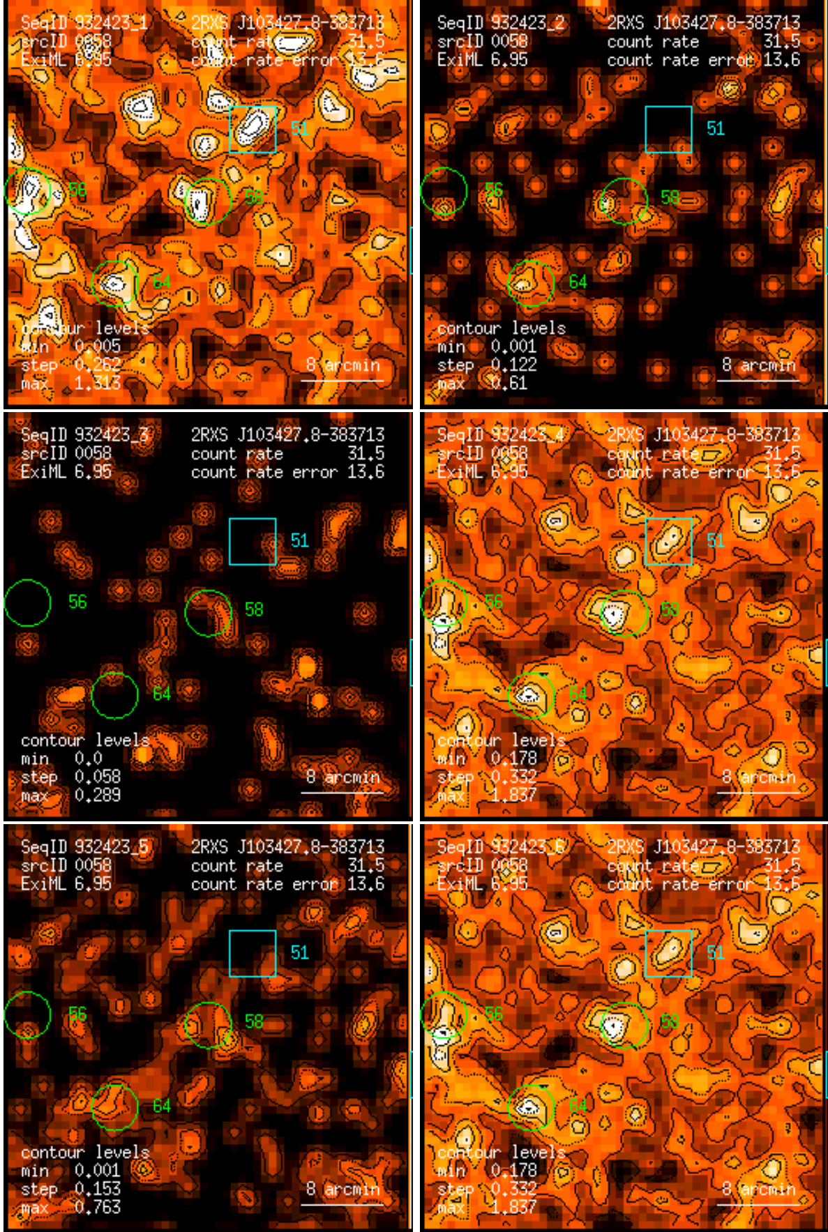
Figure 58: RASS 932423: detection 0058: band rate images, Gaussian filter: (1) PSPC channels 11 – 41, (2) 52 – 90, (3) 91 – 201, (4) 11 – 235, (5) 52 – 201, (6) 11 – 201. Broad band rates in counts/ks. Band rate contour levels in counts/ks/arcmin 2 .
