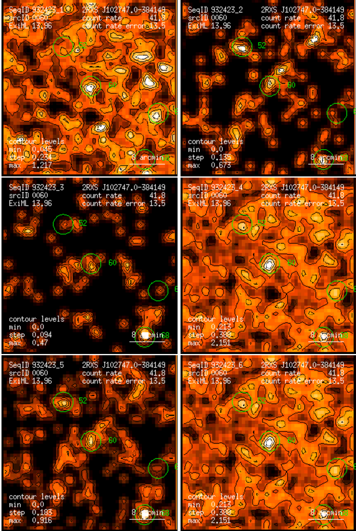
Figure 60: RASS 932423: detection 0060: band rate images, Gaussian filter: (1) PSPC channels 11 – 41, (2) 52 – 90, (3) 91 – 201, (4) 11 – 235, (5) 52 – 201, (6) 11 – 201. Broad band rates in counts/ks. Band rate contour levels in counts/ks/arcmin 2 .
