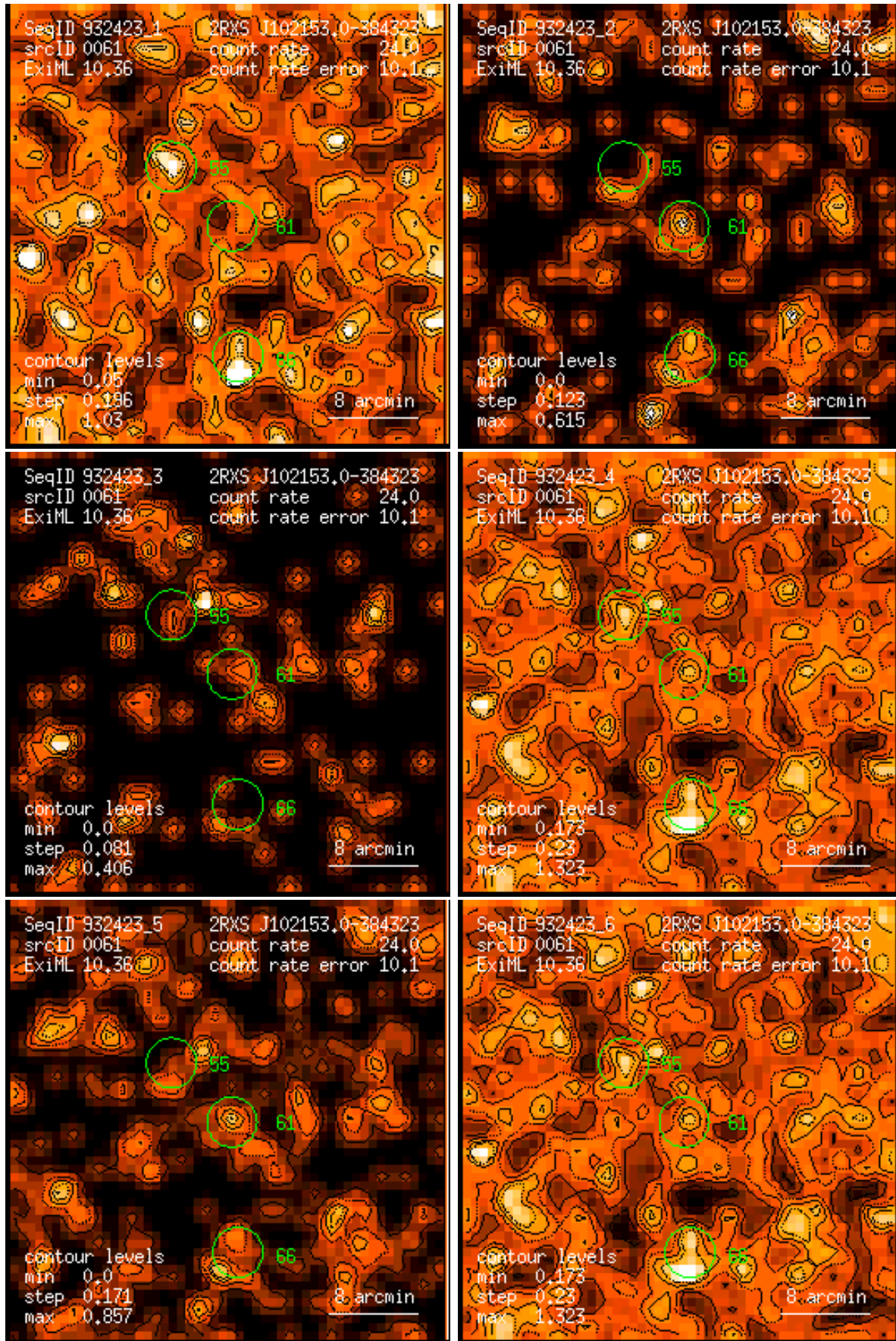
Figure 61: RASS 932423: detection 0061: band rate images, Gaussian filter: (1) PSPC channels 11 – 41, (2) 52 – 90, (3) 91 – 201, (4) 11 – 235, (5) 52 – 201, (6) 11 – 201. Broad band rates in counts/ks. Band rate contour levels in counts/ks/arcmin 2 .
