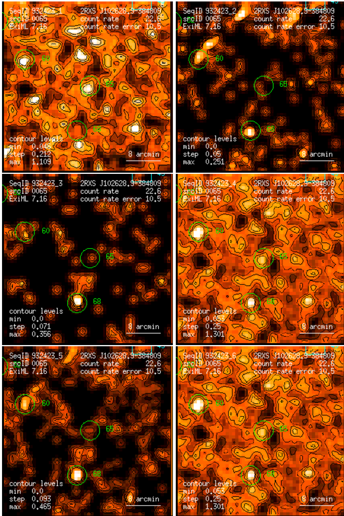
Figure 65: RASS 932423: detection 0065: band rate images, Gaussian filter: (1) PSPC channels 11 – 41, (2) 52 – 90, (3) 91 – 201, (4) 11 – 235, (5) 52 – 201, (6) 11 – 201. Broad band rates in counts/ks. Band rate contour levels in counts/ks/arcmin 2 .
