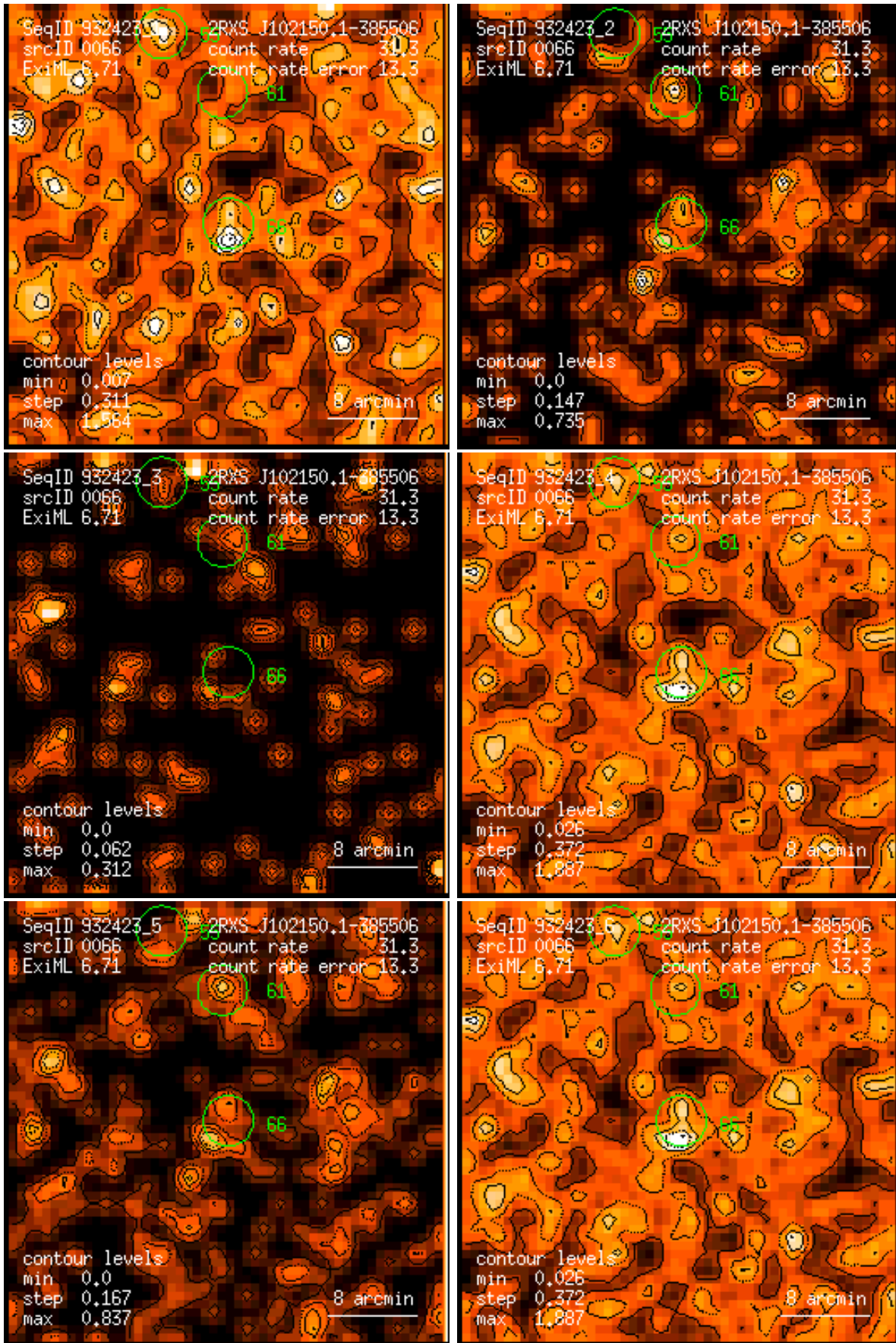
Figure 66: RASS 932423: detection 0066: band rate images, Gaussian filter: (1) PSPC channels 11 – 41, (2) 52 – 90, (3) 91 – 201, (4) 11 – 235, (5) 52 – 201, (6) 11 – 201. Broad band rates in counts/ks. Band rate contour levels in counts/ks/arcmin 2 .
