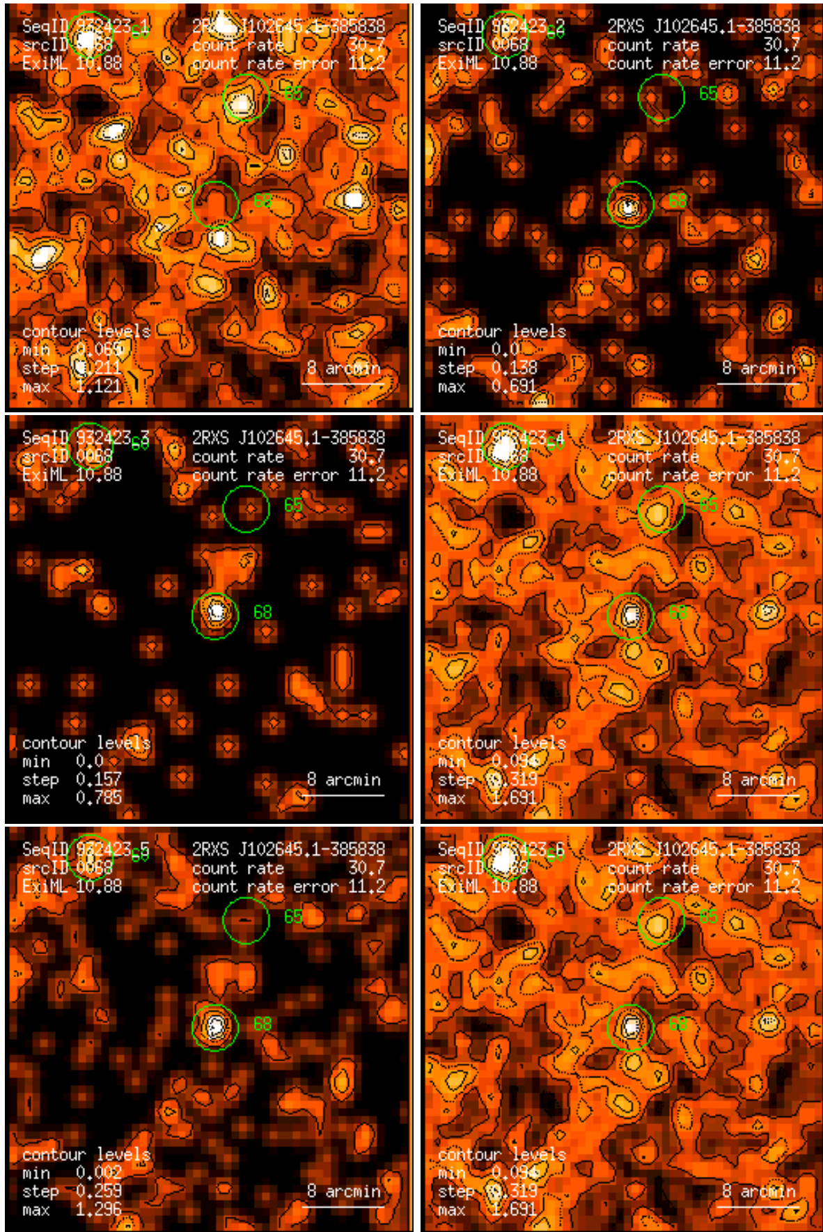
Figure 68: RASS 932423: detection 0068: band rate images, Gaussian filter: (1) PSPC channels 11 – 41, (2) 52 – 90, (3) 91 – 201, (4) 11 – 235, (5) 52 – 201, (6) 11 – 201. Broad band rates in counts/ks. Band rate contour levels in counts/ks/arcmin 2 .
