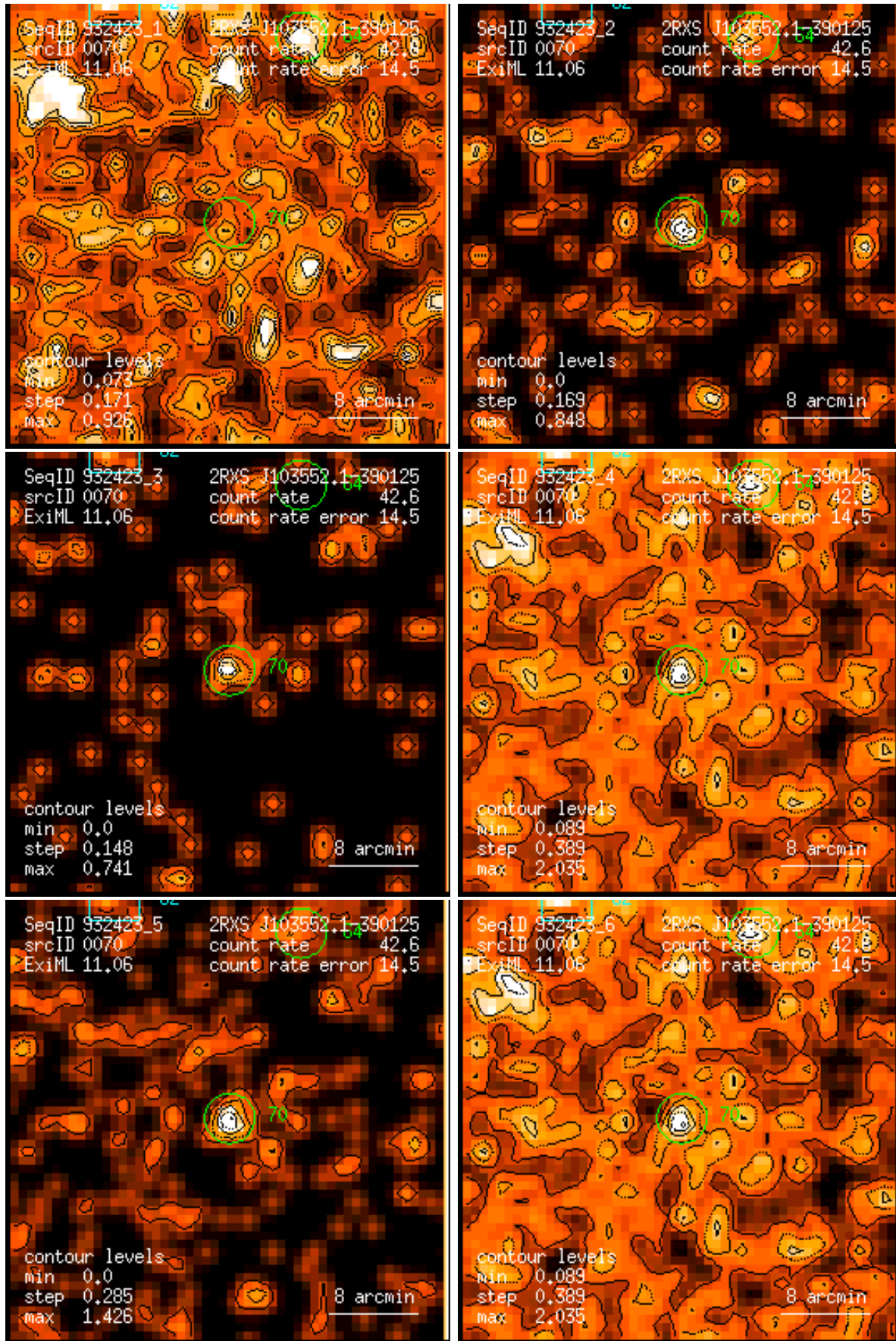
Figure 70: RASS 932423: detection 0070: band rate images, Gaussian filter: (1) PSPC channels 11 – 41, (2) 52 – 90, (3) 91 – 201, (4) 11 – 235, (5) 52 – 201, (6) 11 – 201. Broad band rates in counts/ks. Band rate contour levels in counts/ks/arcmin 2 .
