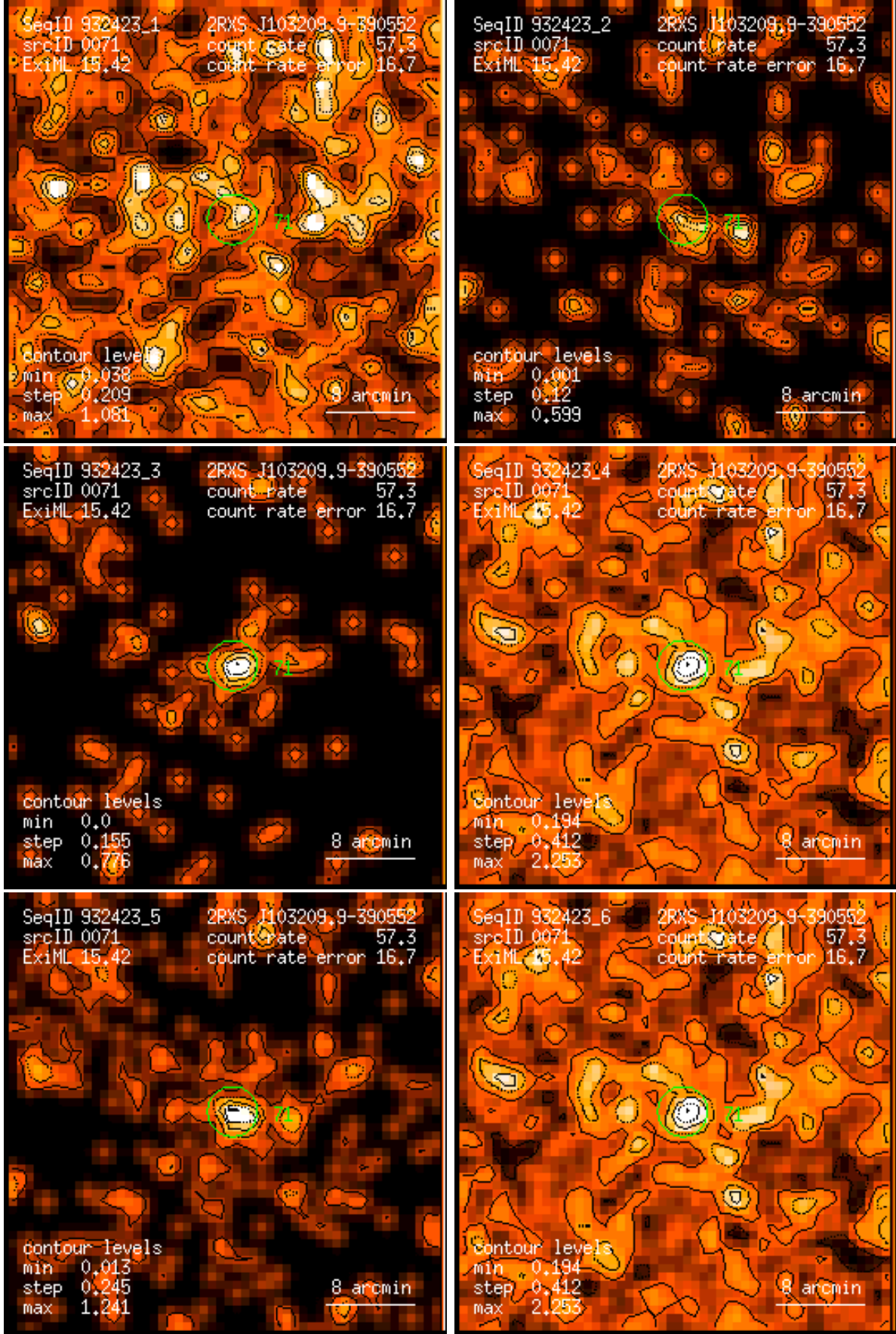
Figure 71: RASS 932423: detection 0071: band rate images, Gaussian filter: (1) PSPC channels 11 – 41, (2) 52 – 90, (3) 91 – 201, (4) 11 – 235, (5) 52 – 201, (6) 11 – 201. Broad band rates in counts/ks. Band rate contour levels in counts/ks/arcmin 2 .
