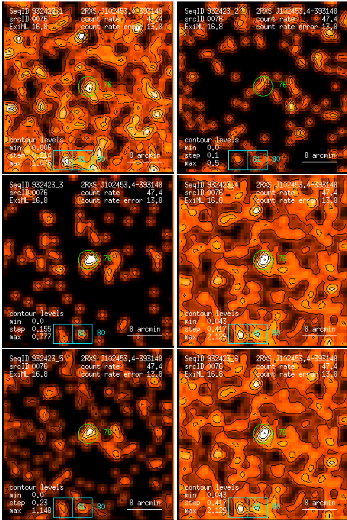
Figure 76: RASS 932423: detection 0076: band rate images, Gaussian filter: (1) PSPC channels 11 – 41, (2) 52 – 90, (3) 91 – 201, (4) 11 – 235, (5) 52 – 201, (6) 11 – 201. Broad band rates in counts/ks. Band rate contour levels in counts/ks/arcmin 2 .
