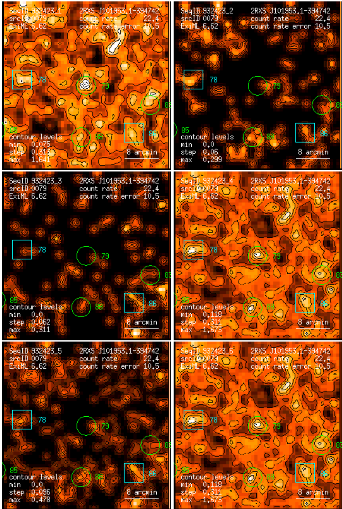
Figure 79: RASS 932423: detection 0079: band rate images, Gaussian filter: (1) PSPC channels 11 – 41, (2) 52 – 90, (3) 91 – 201, (4) 11 – 235, (5) 52 – 201, (6) 11 – 201. Broad band rates in counts/ks. Band rate contour levels in counts/ks/arcmin 2 .
