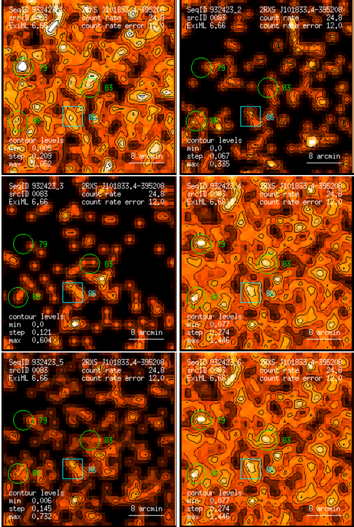
Figure 83: RASS 932423: detection 0083: band rate images, Gaussian filter: (1) PSPC channels 11 – 41, (2) 52 – 90, (3) 91 – 201, (4) 11 – 235, (5) 52 – 201, (6) 11 – 201. Broad band rates in counts/ks. Band rate contour levels in counts/ks/arcmin 2 .
