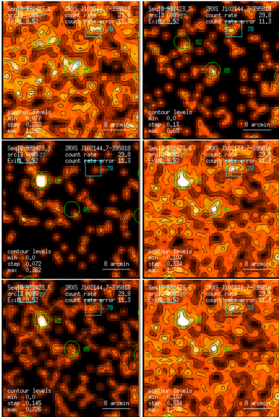
Figure 85: RASS 932423: detection 0085: band rate images, Gaussian filter: (1) PSPC channels 11 – 41, (2) 52 – 90, (3) 91 – 201, (4) 11 – 235, (5) 52 – 201, (6) 11 – 201. Broad band rates in counts/ks. Band rate contour levels in counts/ks/arcmin 2 .
