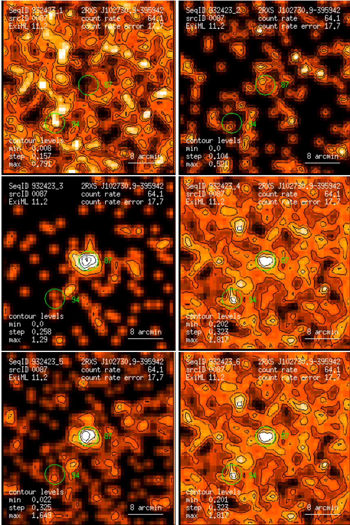
Figure 87: RASS 932423: detection 0087: band rate images, Gaussian filter: (1) PSPC channels 11 – 41, (2) 52 – 90, (3) 91 – 201, (4) 11 – 235, (5) 52 – 201, (6) 11 – 201. Broad band rates in counts/ks. Band rate contour levels in counts/ks/arcmin 2 .
