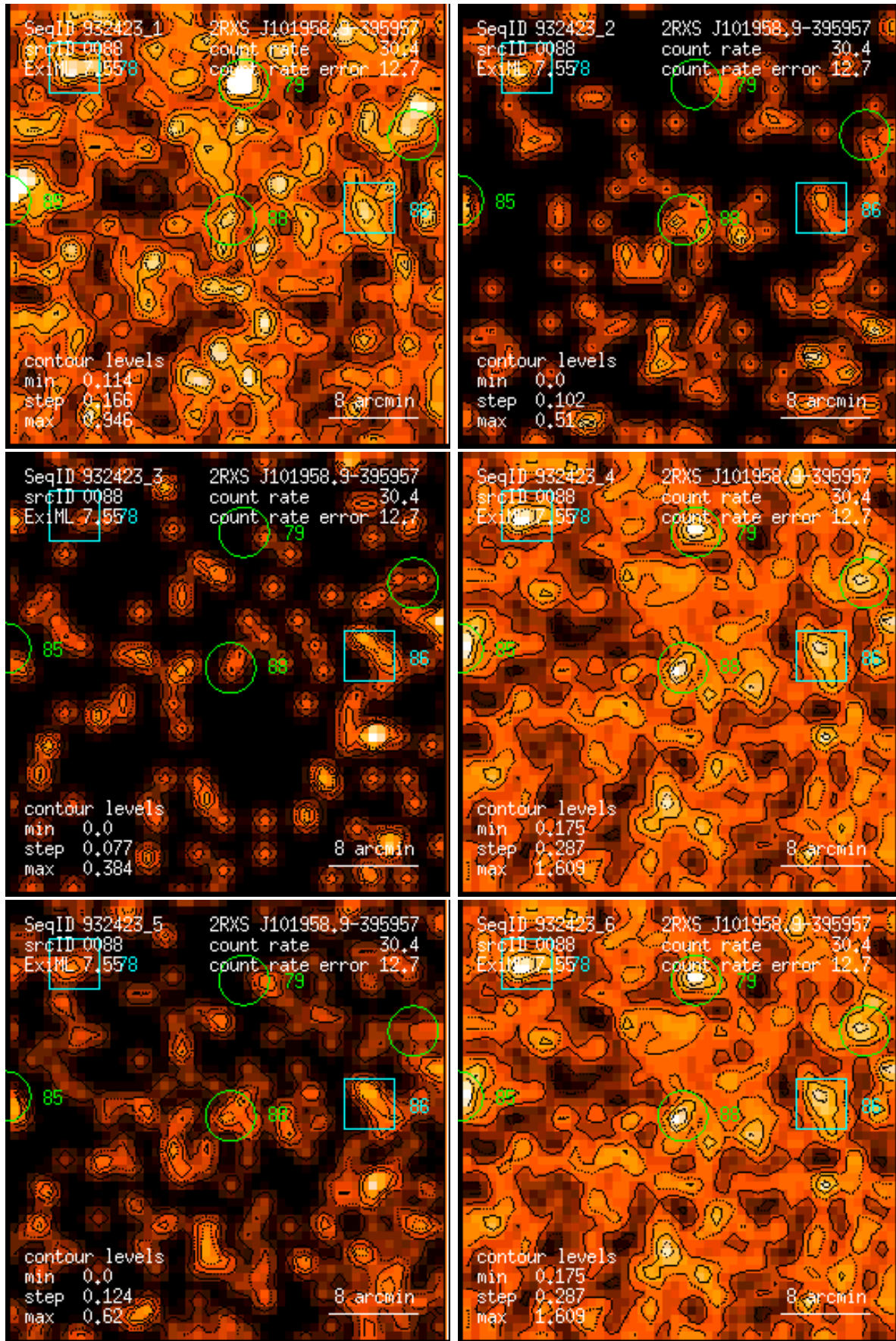
Figure 88: RASS 932423: detection 0088: band rate images, Gaussian filter: (1) PSPC channels 11 – 41, (2) 52 – 90, (3) 91 – 201, (4) 11 – 235, (5) 52 – 201, (6) 11 – 201. Broad band rates in counts/ks. Band rate contour levels in counts/ks/arcmin 2 .
