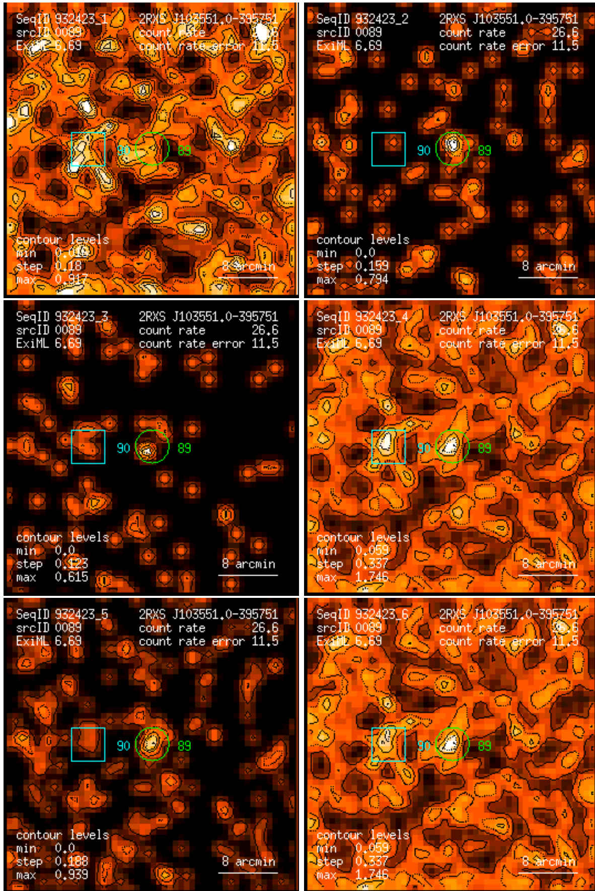
Figure 89: RASS 932423: detection 0089: band rate images, Gaussian filter: (1) PSPC channels 11 – 41, (2) 52 – 90, (3) 91 – 201, (4) 11 – 235, (5) 52 – 201, (6) 11 – 201. Broad band rates in counts/ks. Band rate contour levels in counts/ks/arcmin 2 .
