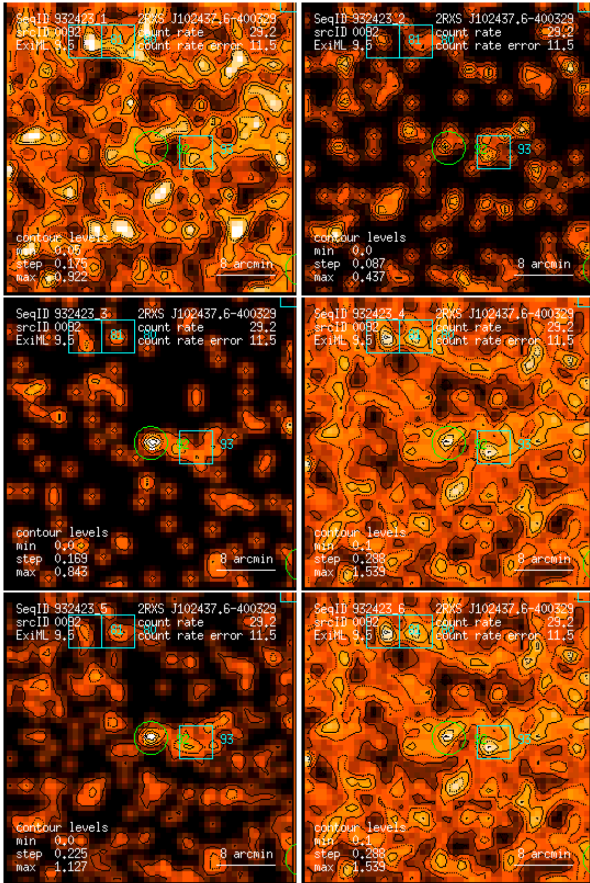
Figure 92: RASS 932423: detection 0092: band rate images, Gaussian filter: (1) PSPC channels 11 – 41, (2) 52 – 90, (3) 91 – 201, (4) 11 – 235, (5) 52 – 201, (6) 11 – 201. Broad band rates in counts/ks. Band rate contour levels in counts/ks/arcmin 2 .
