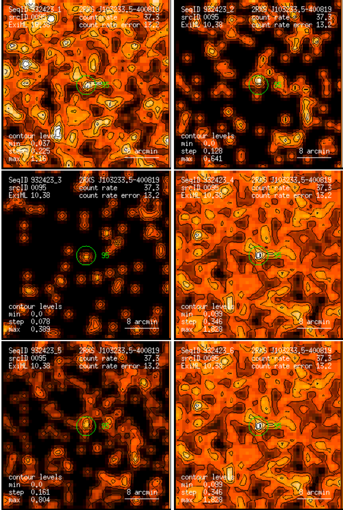
Figure 95: RASS 932423: detection 0095: band rate images, Gaussian filter: (1) PSPC channels 11 – 41, (2) 52 – 90, (3) 91 – 201, (4) 11 – 235, (5) 52 – 201, (6) 11 – 201. Broad band rates in counts/ks. Band rate contour levels in counts/ks/arcmin 2 .
