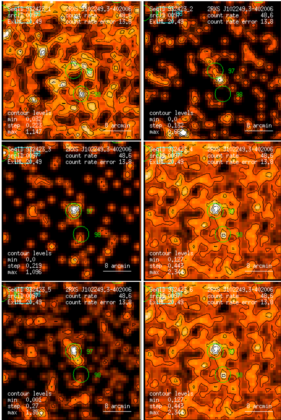
Figure 97: RASS 932423: detection 0097: band rate images, Gaussian filter: (1) PSPC channels 11 – 41, (2) 52 – 90, (3) 91 – 201, (4) 11 – 235, (5) 52 – 201, (6) 11 – 201. Broad band rates in counts/ks. Band rate contour levels in counts/ks/arcmin 2 .
