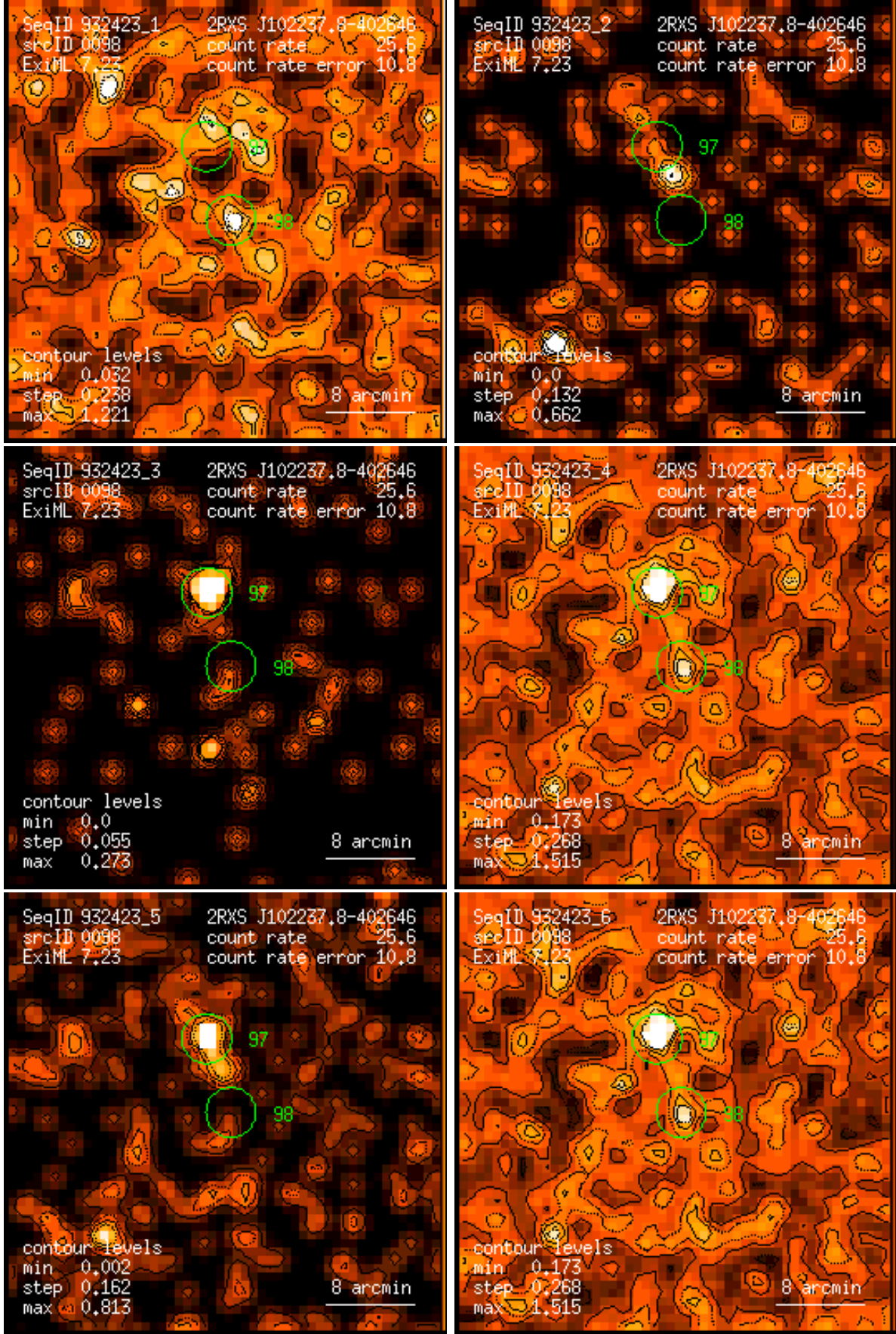
Figure 98: RASS 932423: detection 0098: band rate images, Gaussian filter: (1) PSPC channels 11 – 41, (2) 52 – 90, (3) 91 – 201, (4) 11 – 235, (5) 52 – 201, (6) 11 – 201. Broad band rates in counts/ks. Band rate contour levels in counts/ks/arcmin 2 .
